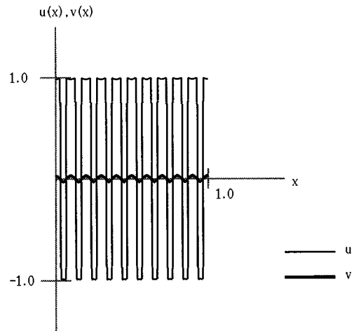
FIG. 2. Shape of the global minimizer as m=0.25 .
