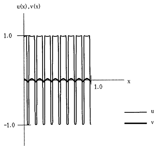
FIG. 3. Shape of the global minimizer as m=0.5 .
