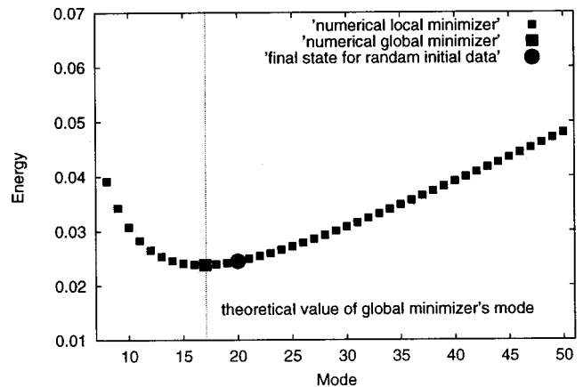
FIG. 7. The mode-energy graph of stable stationary states as m=0.50 .
