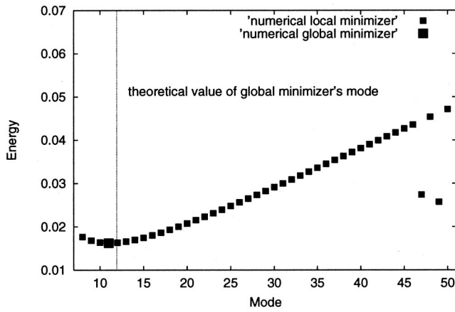
FIG. 8. The mode-energy graph of stable stationary states as m=0.75 .
