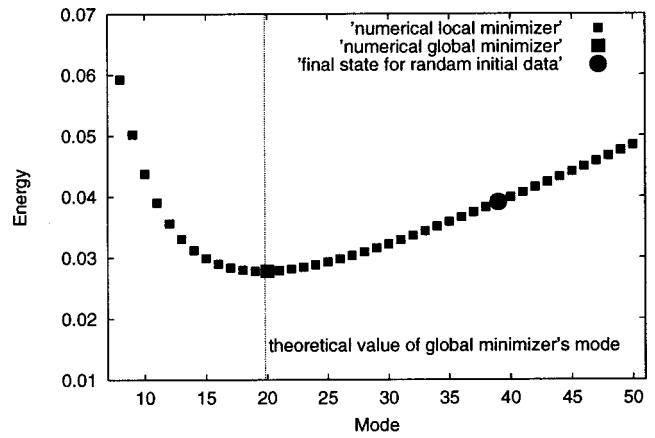
FIG. 6. The mode-energy graph of stable stationary states as m=0.25 .
