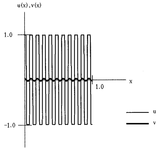
FIG. 1. Shape of the global minimizer as m = 0.0 .
