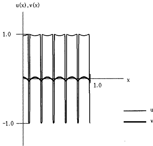
FIG. 4. Shape of the global minimizer as m=0.75 .
