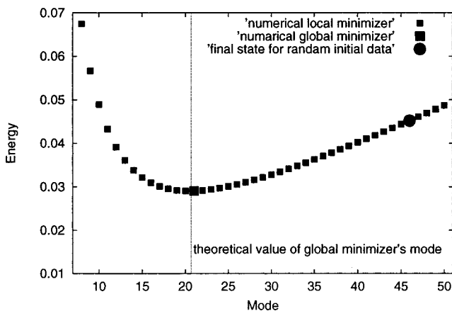
FIG. 5. The mode-energy graph of stable stationary states as m=0.0 .
