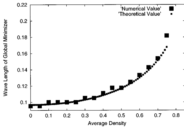
FIG. 9. The m -wavelength graph as \varepsilon=0.001 and \sigma=100 .
