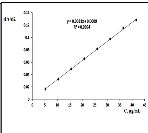
Fig. 5: Calibration curve for (Dapagliflozin Propanediol .H 2 O)
