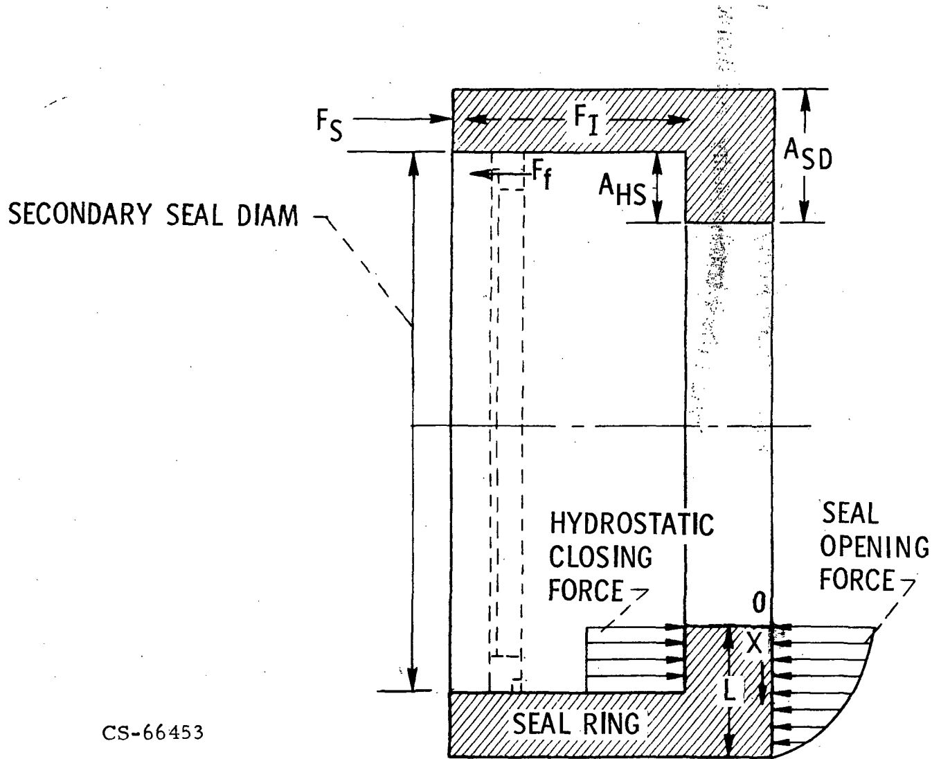
Figure 2. - Schematic of radial face seal identifying the nomenclature.
