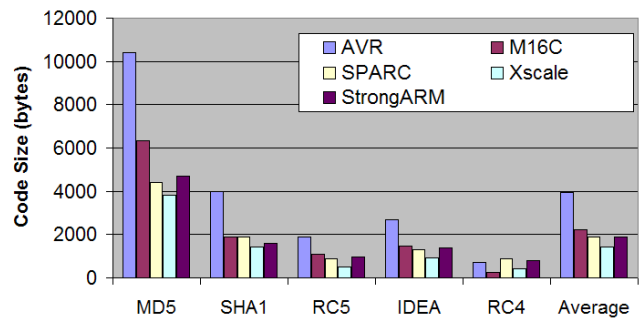
Figure 4: Code sizes for algorithms
