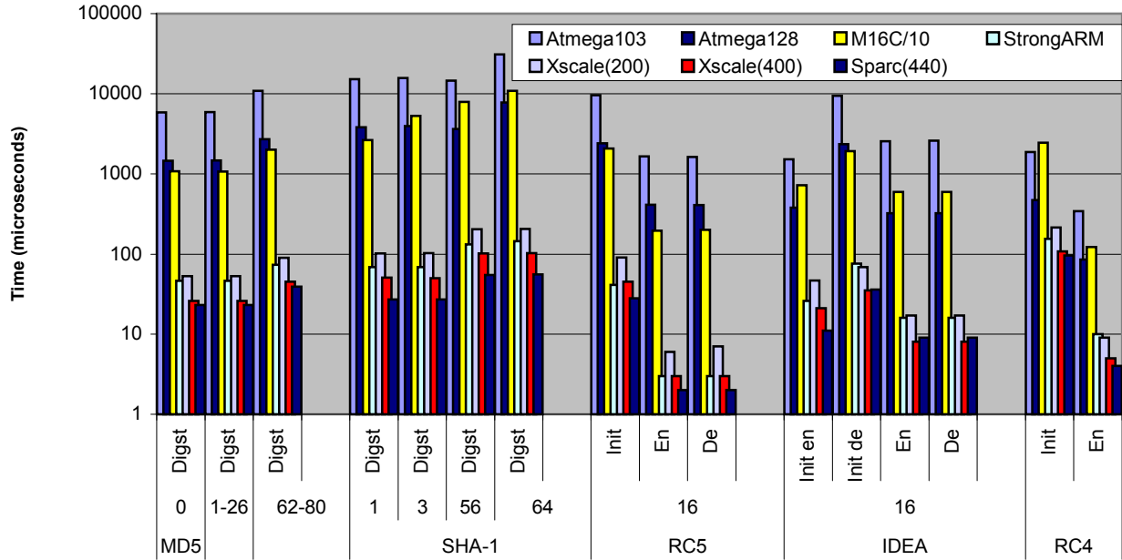
Figure 1: Execution times [μs] for algorithms, platforms and plaintext sizes [bytes]
