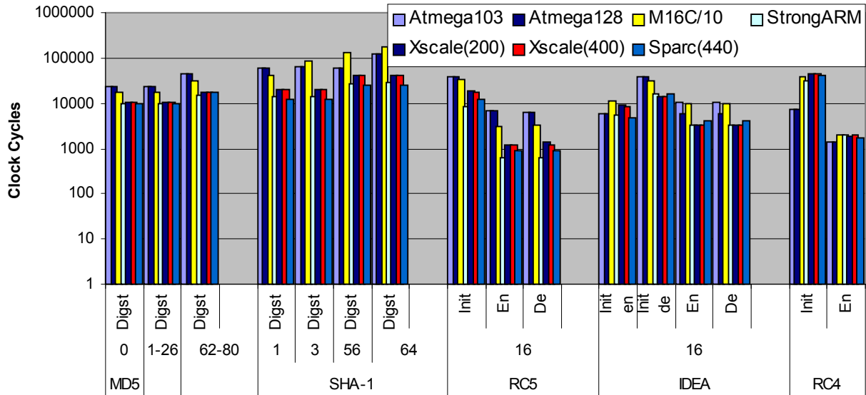
Figure 2: Clock cycles for algorithms, platforms and various plaintext sizes [bytes]
