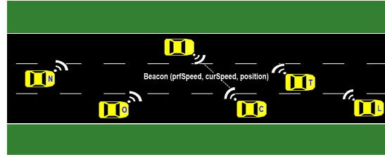
Fig. 2: Exchange of vicinity attributes using beacons
