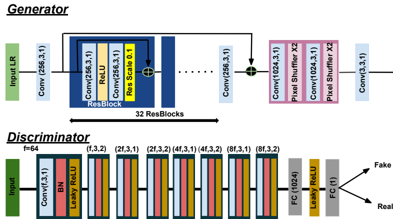
Fig. 1. Network architecture of EPSR.
