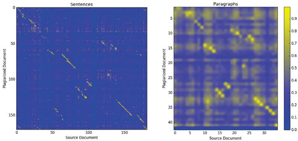
Figure 3: Heatmap of semantic relatedness scores in a plagiarized document and its source.
