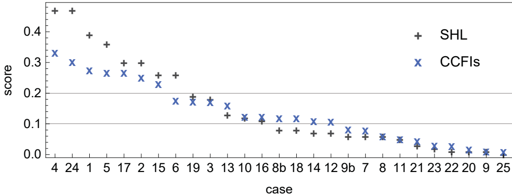
Figure 4: Similarity scores of Sherlock and CCFI_s for all source documents.
