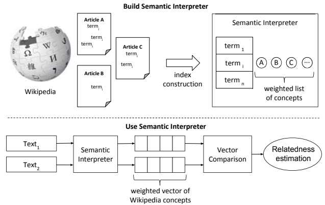
Figure 1: Concept of Explicit Semantic Analysis [13].
