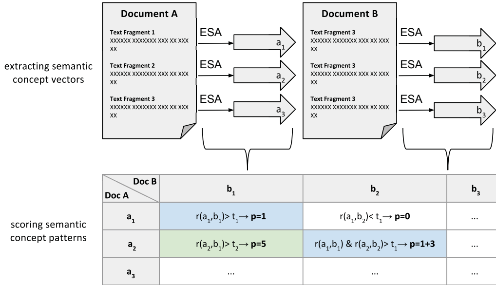
Figure 2: Semantic Sequence Scoring (variant SSS_a ).
