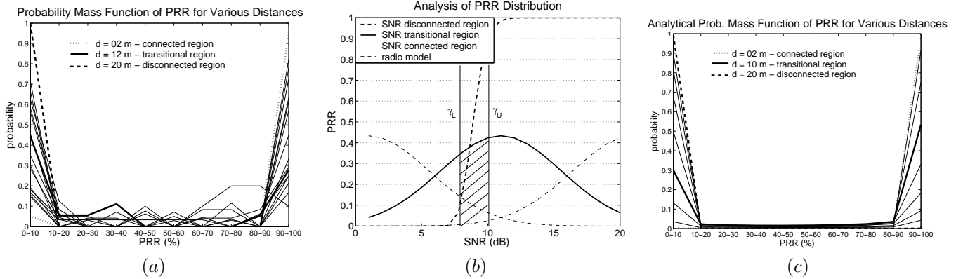
Fig. 13. PRR Distribution for Different Transmitter-Receiver Distances. (a) empirical distribution of the high-power-outdoor environment, (b) analytical observation of the distribution, (c) analytical distribution of the high-power-outdoor environment
