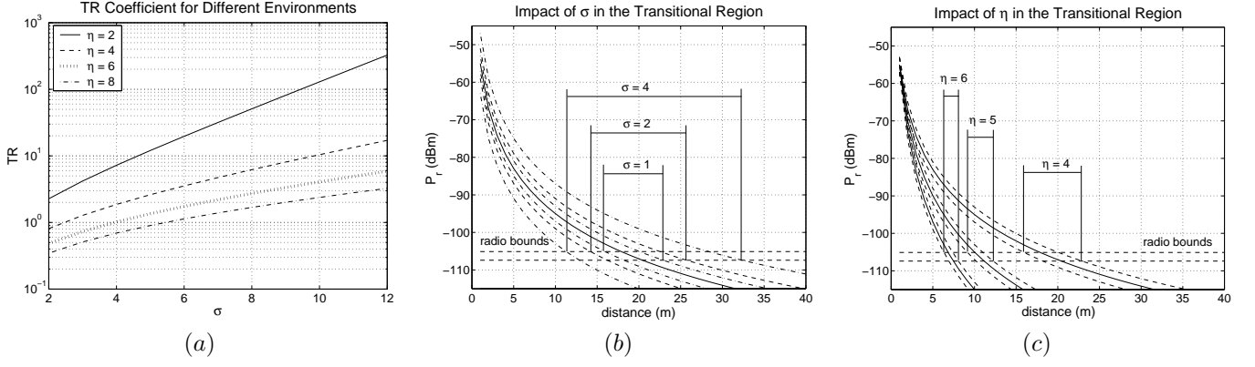
Fig. 5. Impact of the path loss exponent n and the log-normal shadowing standard deviation \sigma on the Transitional Region. (a) \Gamma coefficient for various \sigma and n . (b) if \sigma increases, the transitional region increases. (c) if n increases, the transitional region decreases
