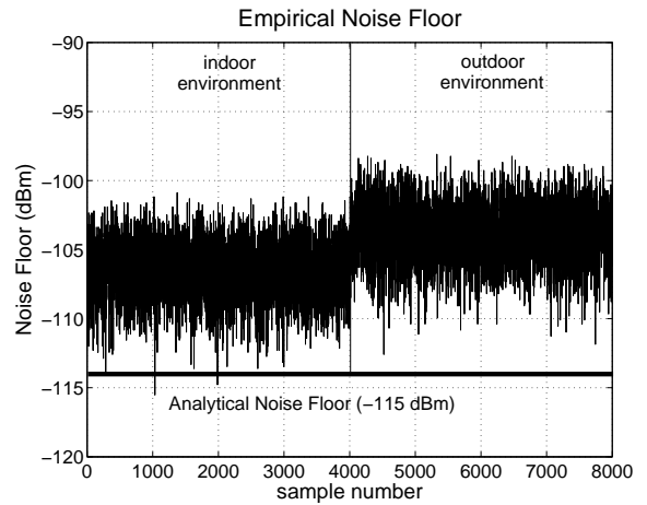
Fig. 9. Empirical Measurements of the Noise Floor.
