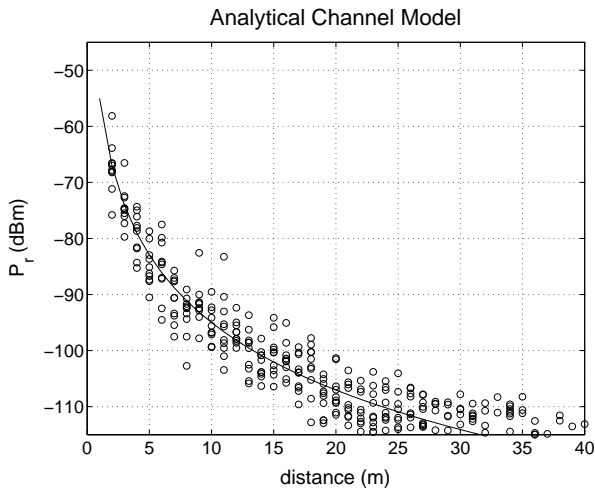
Fig. 1. Channel Model, n = 4 , \sigma = 4 , P_t = 0 dBm
