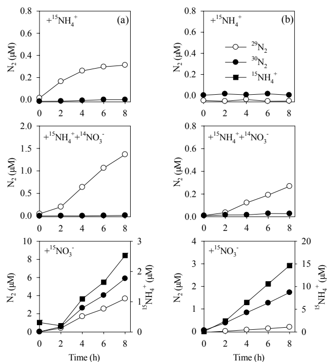
Fig. 3. Production of ^{29}\text{N}_2 , ^{30}\text{N}_2 and ^{15}\text{NH}_4^+ against time in slurry incubation. (a) DH31 0–2 cm sediment. The residual nitrate was not exhausted after the 24 h pre-incubation, thus we observed a slight ^{29}\text{N}_2 production before all the nitrate disappeared; (b) DH15 6–8 cm sediment. The nitrate was less than 1 \mu\text{M} after pre-incubation, hence we did not detect significant ^{29}\text{N}_2 production.
