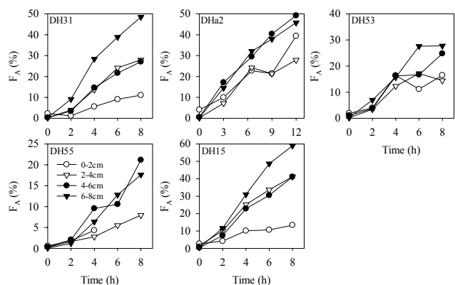
Fig. 4. Time course of ^{15}\text{NH}_4^+ fraction ( F_A ) in E_Denit.
