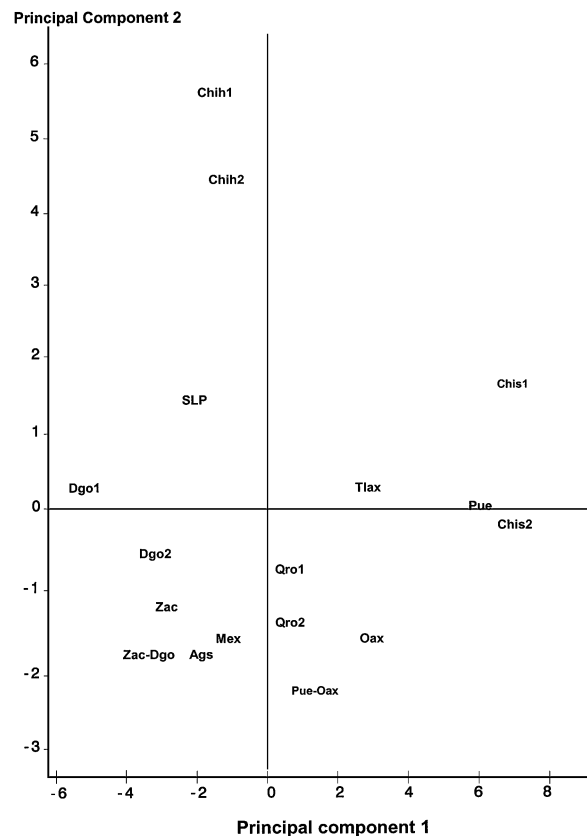
Fig. 4. Principal component analysis based on wood, climate, and soil variables, plotted for provenances where individuals of B. cordata were collected; see Table 1 for provenance information. Provenances: Chih1 = Chihuahua 1, Chih2 = Chihuahua 2, Dgo1 = Durango 1, Dgo2 = Durango 2, Dgo-Zac = Durango-Zacatecas, Zac = Zacatecas, Ags = Aguascalientes, SLP = San Luis Potosí, Qro1 = Queretaro 1, Qro2 = Queretaro 2, Tlax = Tlaxcala, Mex = Mexico, Pue = Puebla, Pue-Oax = Puebla-Oaxaca, Chis1 = Chiapas 1, Chis2 = Chiapas 2
