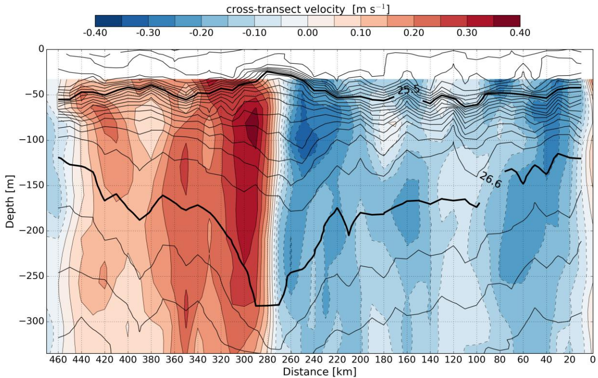
Figure 2: Vertical section along the east-west transect in Phase 1 (3-5 September 2014; Figure 1, green line) of the cross-transect ADCP velocity with superimposed contours of potential density anomaly, \sigma_\theta . Thick contours are \sigma_\theta = 25.5 \text{ kg m}^{-3} and \sigma_\theta = 26.6 \text{ kg m}^{-3} (contour interval is 0.1 \text{ kg m}^{-3} ).
