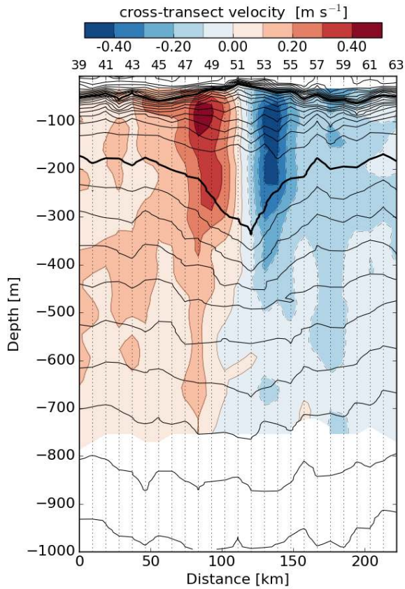
Figure 3: Vertical section of the cross-transect (zonal) ADCP velocity (positive values indicate eastward velocity and negative values indicate westward velocity) along the Le Tourmalet meridional transect (12-15 September 2014; Figure 1, white stars) with superimposed contours of potential density anomaly, \sigma_\theta . Thick contours indicate \sigma_\theta = 25.5 \text{kg m}^{-3} and \sigma_\theta = 26.6 \text{kg m}^{-3} (contour interval is 0.1 \text{kg m}^{-3} ). Vertical dotted lines show the CTD station positions, only odd station numbers are included for clarity.
