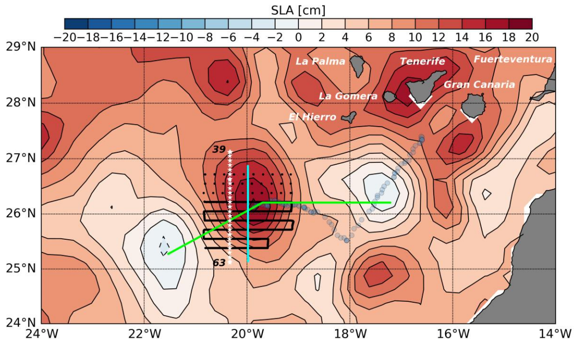
Figure 1: Map of the Eddy Canary Corridor. Colors show sea level anomaly (SLA) from AVISO on 3 September 2014. Green and cyan lines represent Phase 1 of the PUMP cruise, taken to locate the eddy center. Black lines and dots mark the grid of the 3D eddy sample with SeaSoar continuous tows and rosette system discrete casts, respectively (Phase 2). White stars indicate high-resolution CTD stations in Le Tourmalet section (Phase 3). The trajectory of the eddy center from its formation to the beginning of the cruise is depicted by blue dots (the time interval between dots is 1 day). The eddy translated westwards with a speed of 4 \text{ km d}^{-1} ( 0.046 \text{ m s}^{-1} ) during the eddy sampling.
