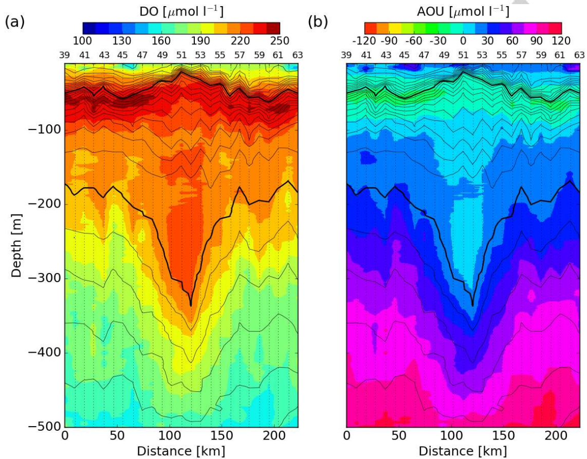
Figure 5: Vertical sections of (a) Dissolved oxygen (DO) and (b) apparent oxygen utilization (AOU) along the Le Tourmalet transect (Figure 1, white stars). Contours represent potential density anomaly, \sigma_{\theta} . Thick contours are the 25.5 \text{ kg m}^{-3} and 26.6 \text{ kg m}^{-3} isopycnals (contour interval is 0.1 \text{ kg m}^{-3} ).
