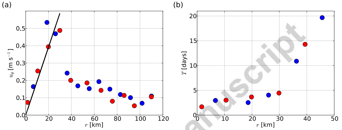
Figure 10: Radial sections of absolute azimuthal velocity, u_\theta , (a) and orbital period (b) for the Le Tourmalet transect (Figure 1, white stars). Sections are taken at the depth of maximum azimuthal velocity (97 m for the Le Tourmalet transect). Solid line in (a) shows the linear fit u_\theta = \omega_0 r , with \omega_0 = 1.96 \cdot 10^{-5} \text{ s}^{-1} (angular velocity). (b) Represents the radial distribution of the orbital period computed as 2\pi r/u_\theta . Red and blue dots represent u_\theta and T positions north and south of the eddy center, respectively.
