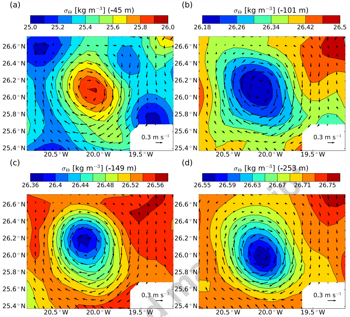
Figure 6: Objectively mapped ADCP velocity vectors with \sigma_\theta contours at different depths. Correlation scales used in the objectively interpolation are L_x = L_y = 40 km and the uncorrelated noise applied is 3%.
