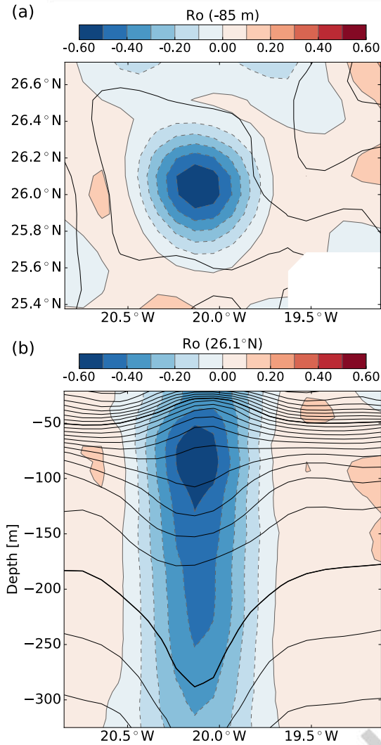
Figure 9: (a) Rossby number, Ro , horizontal distribution at 85 m depth. (b) Ro zonal section along 26.1^\circ\text{N} . Black contours indicate the objectively mapped \sigma_\theta , with a contour interval of 0.1 \text{ kg m}^{-3} . Thick contours are the 25.5 \text{ kg m}^{-3} and 26.6 \text{ kg m}^{-3} isopycnals.
