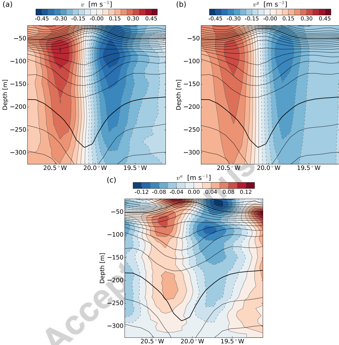
Figure 7: Vertical distributions of the meridional components of the (a) objectively mapped ADCP velocity, v , (b) geostrophic velocity, v^g , and (c) ageostrophic velocity, v^a = v - v^g , along 26.1°N. Black contours correspond to the objectively mapped potential density anomaly ( \sigma_\theta , with a contour interval of 0.1 kg m -3 ). Thick contours are the 25.5 kg m -3 and 26.6 kg m -3 isopycnals. Note different color scale in (c).
