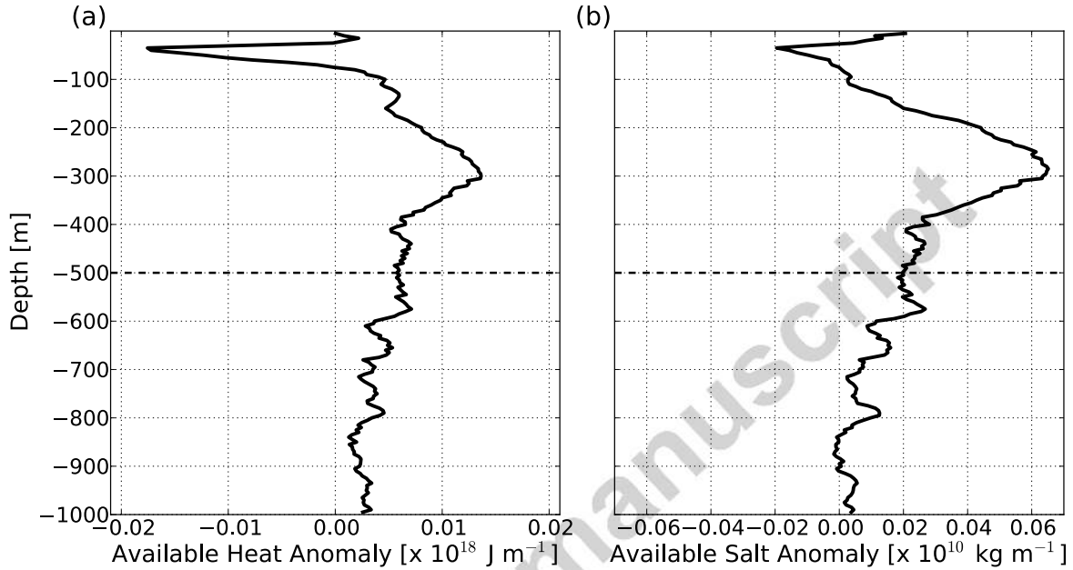
Figure 12: Vertical profiles of the available heat (a) and salt (b) content anomalies transported by the eddy core. Horizontal dashed lines represent the eddy base.
