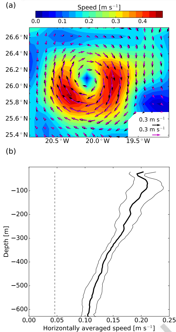
Figure 8: (a) ADCP velocity magnitude at 85 m depth. Black arrows represent ADCP velocity vectors whereas magenta arrows correspond to geostrophic velocity vectors. (b) Vertical profile of the horizontally averaged ADCP velocity magnitude (thick black line) with the standard deviation represented by thin black lines. Dashed line indicates the mean translation speed ( 0.046 \text{ m s}^{-1} ).
