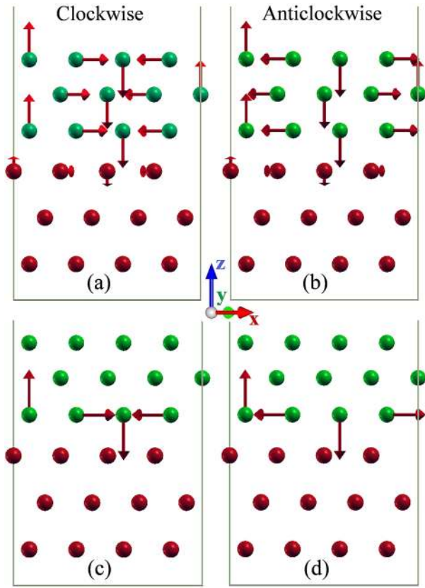
FIG. 1 (color online). Examples of (a),(c) clockwise (CW) and (b),(d) anticlockwise (ACW) spin configurations used to calculate the DMI of hcp(0001)Co/fcc(111)Pt bilayers. The total d^{\text{tot}} and the layer-resolved d^k DMI parameters were found using (a), (b) and (c),(d) spiral configurations, respectively (see the text). Green and red correspond respectively to Co and Pt. Spin moments of Pt atoms are multiplied by 10 for convenience. The side view of the Co(3)Pt(3) unit cell is represented.
