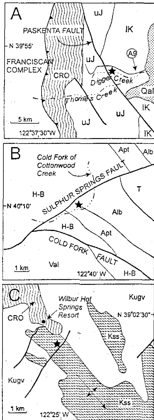
Fig.3. Geology of the three seep-carbonate deposits (stars) of this study. (A) The Paskenta deposit (Tithonian) is situated within a synsedimentary, listric fault zone (Paskenta Fault). Compare with field photograph (Fig.4A). UJ, IK = Upper Jurassic, Lower Cretaceous. Geology modified from Jones et al. (1969). (B) The Cold Fork of Cottonwood Creek site (Albian–Aptian) is situated near the junction of the synsedimentary Cold Fork and Sulphur Springs Faults. Val = Valanginian, H-B = Hauterivian–Barremian; Alb = Albian; Apt = Aptian; T = Tertiary. Map and ages of stratigraphic units modified from Bailey & Jones (1973). (C) The Wilbur Springs deposit (Hauterivian) occurs in diapir-associated sedimentary serpentinites (Kss) affiliated with the Coast Range Ophiolite (CRO) and Great Valley Group turbidites (Kugv). Map simplified from Carlson (1984).
