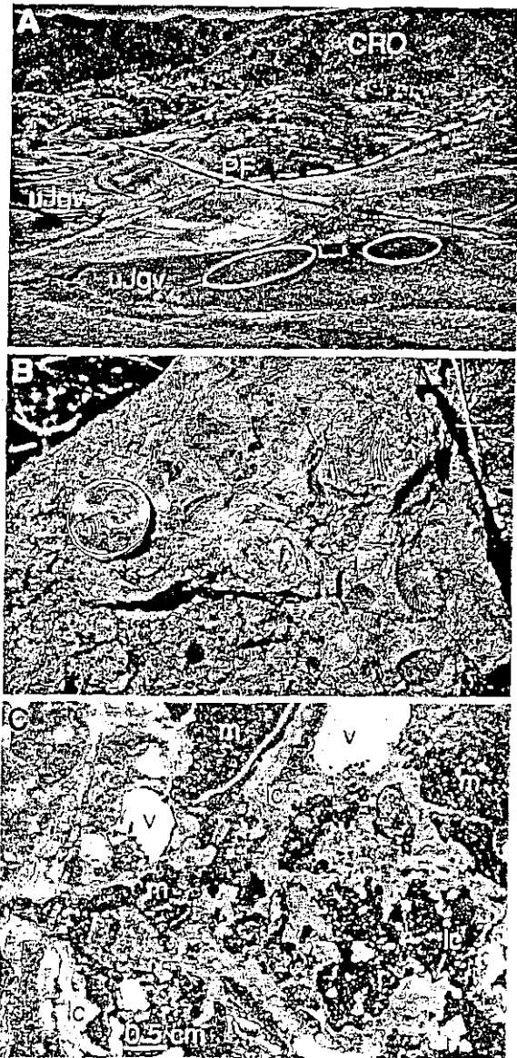
Fig. 4. Typical outcrop, hand sample and broad petrographic characteristics of Mesozoic seep-carbonates, California. (A) Paskenta held locality, situated between Digger Creek (left and foreground) and county road A9; view to west. Illustrated geology includes: isolated seep-carbonate mounds (circles) enclosed by fine-grained slope turbidites of Upper Jurassic Great Valley Group (UJGV), syndimentary Paskenta Fault zone (broken line, PF) and tectonically juxtaposed Coast Range Ophiolite (CRO). (B) Outcrop float block from Wilbur Springs seep-carbonate deposit, characterized by fossil-rich micrite and seep-restricted brachiopod Peregrinella whitneyi (cf. Campbell & Bottjer 1995b). Coin = 1.8 cm in diameter. (C) Entire thin section view (4.0 cm long, PS1-1A) of typical seep-carbonate, broadly divisible into dark micrite (m) and light-coloured cements (lc), separated by dark, irregular, pyrite-coated corrosion surfaces. Clear calcite spar-filled vugs (v) common. Transmitted light.
