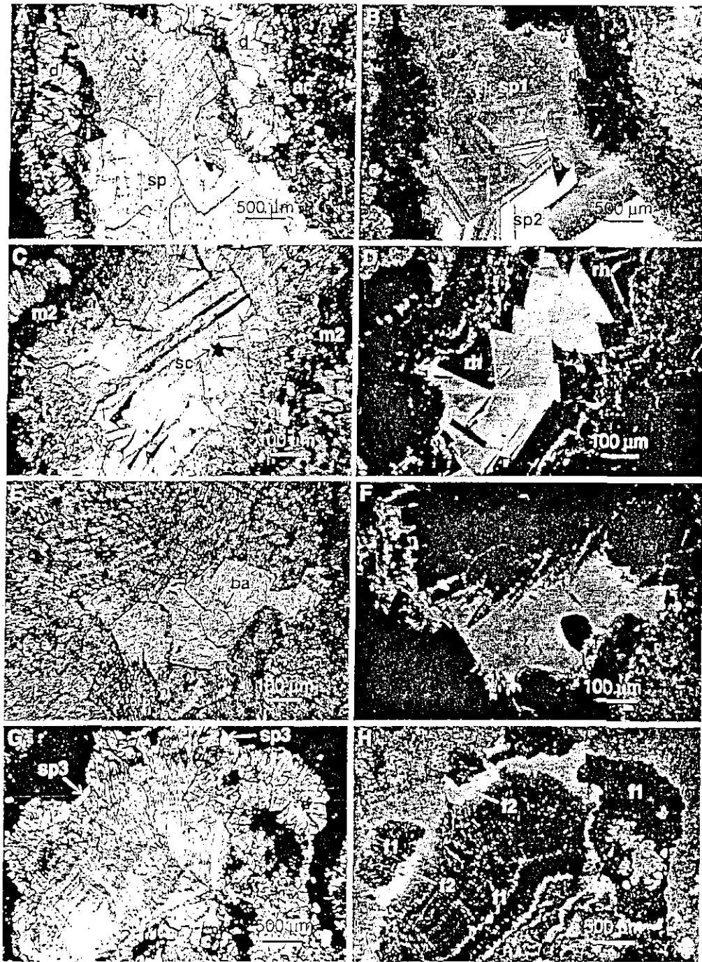
Fig. B. Petrographic aspects of late diagenetic phases. (A) Cavity lined with dentate cement (d), inclusion-rich isopachous cement (i) and blocky calcite spar (sp); dentate cement enclosed remnant acicular fibrous crystals (ac). CC-240-1, plane-polarized light. (B) Same view and magnification as in (A), in CL, displaying nonluminescent character of dentate and acicular fibrous cements, grainy dull orange Ct of isopachous horizons and sectoral zonation of calcite spar – both dark orange (spar 1, sp1) and orange (spar 2, sp2) varieties. (C) Late-stage phases filling pore space in worm tube (CC-240-1), including micrite 2 lining (m2), inclusion-rich isopachous crust (i), blocky calcite spar (sp) and minor rill-clay (sc). Plane-polarized light. (D) Same view as in (C), in CL, revealing rhombohedral calcite (rh) phase not detected in transmitted light, and sectoral zonation of blocky calcite spar. (E) Details of radially fibrous cement and small pore cemented with late, blocky calcite spar and birefringent, prismatic barite crystal (ba). CC-80-5, plane-polarized light. (F) Same view and magnification as in (E), in CL, illuminating fibrous 1 subcrystal tips with laterally adjacent pyramidal and tabular habits, and nonluminescent character of barite. (G) Vug formed in micrite 1, filled with radially fibrous cement, minor moldic porosity (CE3) filled with late spar 3 (sp3). PN1-1A, plane-polarized light. (H) Same view and magnification as in (G), in CL, displaying darkly luminescent, early fibrous cement (f1) cut by band of bright yellow, recrystallized fibrous cement (f2); bright band spatially associated with fenestrae of late spar 3.
