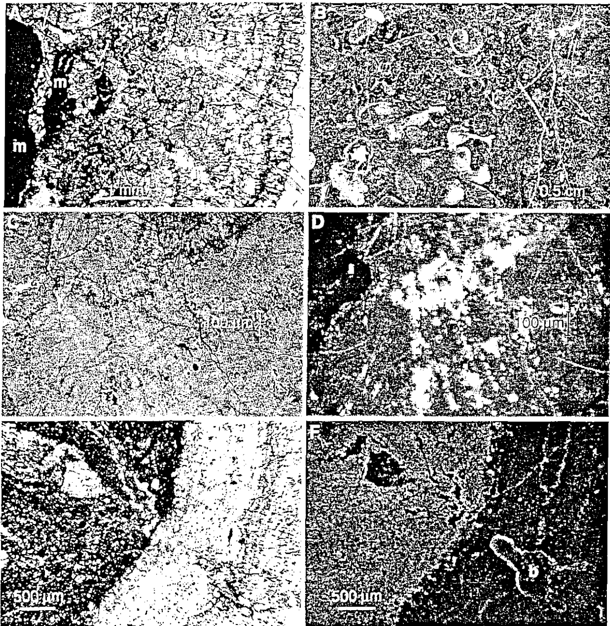
Fig. 7. Petrographic aspects of early events of cement stratigraphy. (A) Early diagenetic sequence (PN1-9A), from micrite 1 ( m ), to first corrosion event (CE1, arrows), to anhedral yellow calcite ( y ), to fibrous 1 cement ( f ). Plane-polarized light. (B) Bioturbated, detrital-rich micrite 1 phase, with gastropods, calcispheres and scattered pyrite grains. Entire thin section view (4.0 cm long, PS1-4A), transmitted light. (C) Transition from anhedral yellow calcite (upper left corner) to fibrous 1 cement, the latter exhibiting brown globules and black streaks inferred as petroleum inclusions (PN1-9A). Plane-polarized light. (D) Same view and magnification as in (C), in UV; hydrocarbon inclusions in the fibrous cement fluoresced bright yellow-green. (E) Micrite 1 overlain by fibrous 1 cement with golden to reddish brown petroleum inclusions (PN1-1D). Plane-polarized light. (F) Same view and magnification as in (E) in CL; marine boring structure ( b , ~1.3 mm long) revealed in lower right corner.
