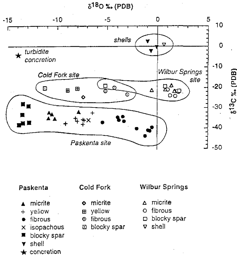
Fig. 11. Stable carbon versus oxygen isotopic cross-plot for Paskenta, Cold Fork of Cottonwood Creek and Wilbur Springs seep-carbonate deposits revealed four distinct fields (encircled).
