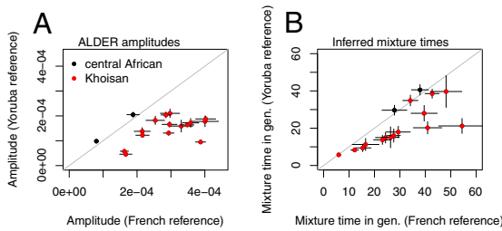
Fig. 2. Relationship with west Eurasia is shared by all Khoisan populations. We generated weighted LD decay curves in each Khoisan (or central African hunter-gatherer) population, using weights computed using the test population as one reference and either the French or the Yoruba as the other reference. We then fit an exponential decay model to each LD curve. Plotted are the inferred (A) amplitudes and (B) admixture times in each population. Larger amplitudes indicate a closer relationship to the true admixing population, and under a model of a single admixture event the admixture times do not depend on the reference populations used.
