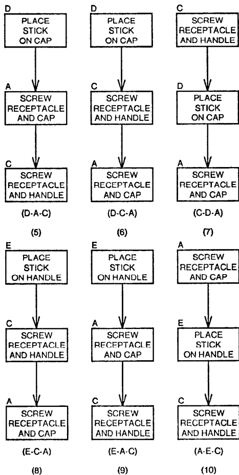
Figure 2: Possible sequences of operations to assemble the product shown in figure 1
