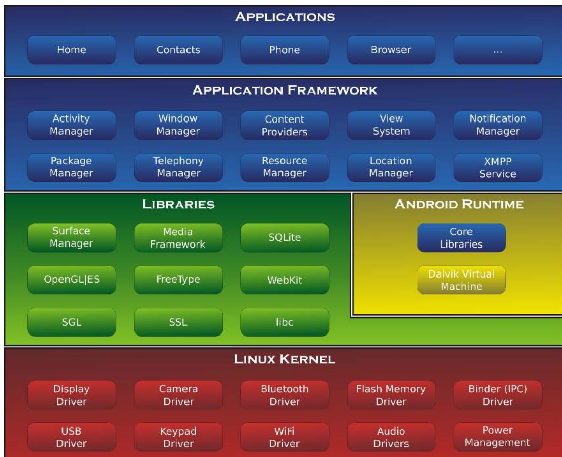
FIGURE 2.1: Android's Stack Structure
