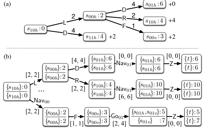
Figure 2: (a) A standard lookahead tree for our example. Nodes are labeled with states (written s_{xy(h/v)} ) and costs-so-far, edges are labeled with actions and associated costs, and leaves have a heuristic estimate of the remaining distance-to-goal. (b) An abstract lookahead tree (ALT) for our example. Nodes are labeled with optimistic and pessimistic simple valuations and edges are labeled with (possibly high-level) actions and associated optimistic and pessimistic costs.
