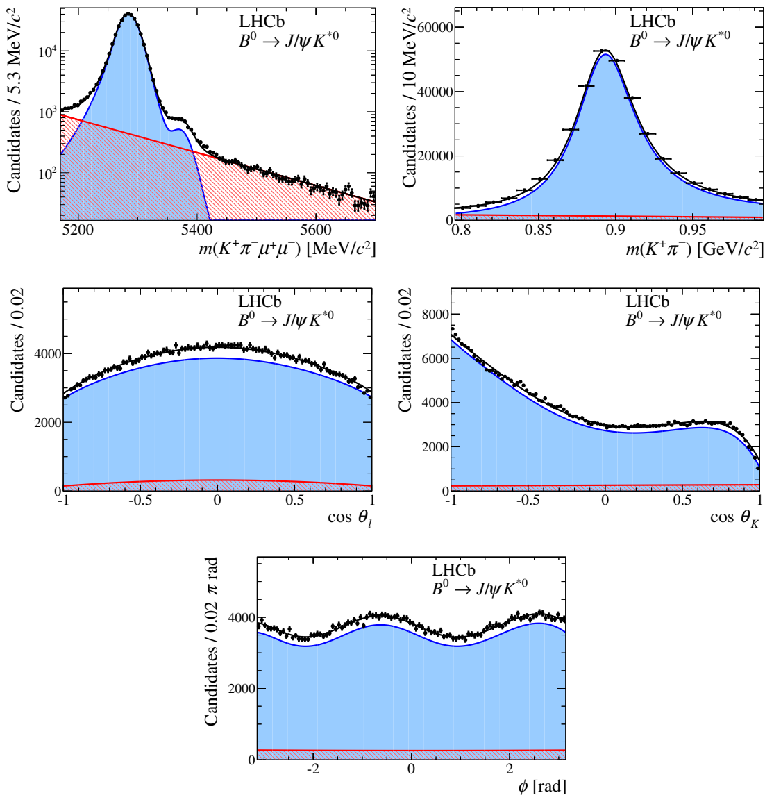
Figure 15. Angular and mass distribution of B^0 \rightarrow J/\psi K^{*0} candidates in data. A small signal component is also included in the fit to account for B_s^0 \rightarrow J/\psi K^{*0} decays. Overlaid are the projections of the total fitted distribution (black line) and its different components. The signal is shown by the solid blue component and the background by the red hatched component.
