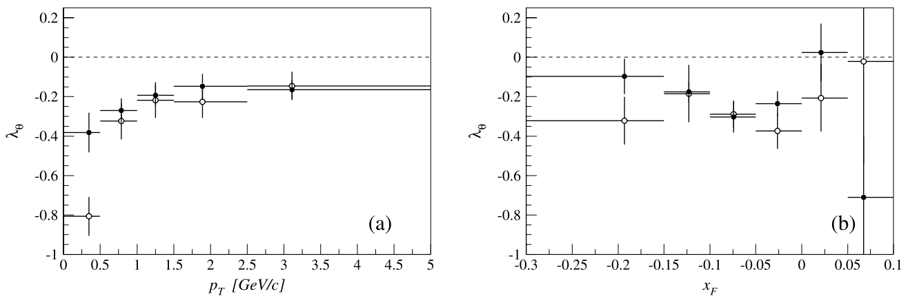
Fig. 3.3 The parameter \lambda_\theta measured in the Collins-Soper frame in carbon (black points) and tungsten (white points) as functions of the average reconstructed p_T (a) and x_F (b). The vertical error bars represent
