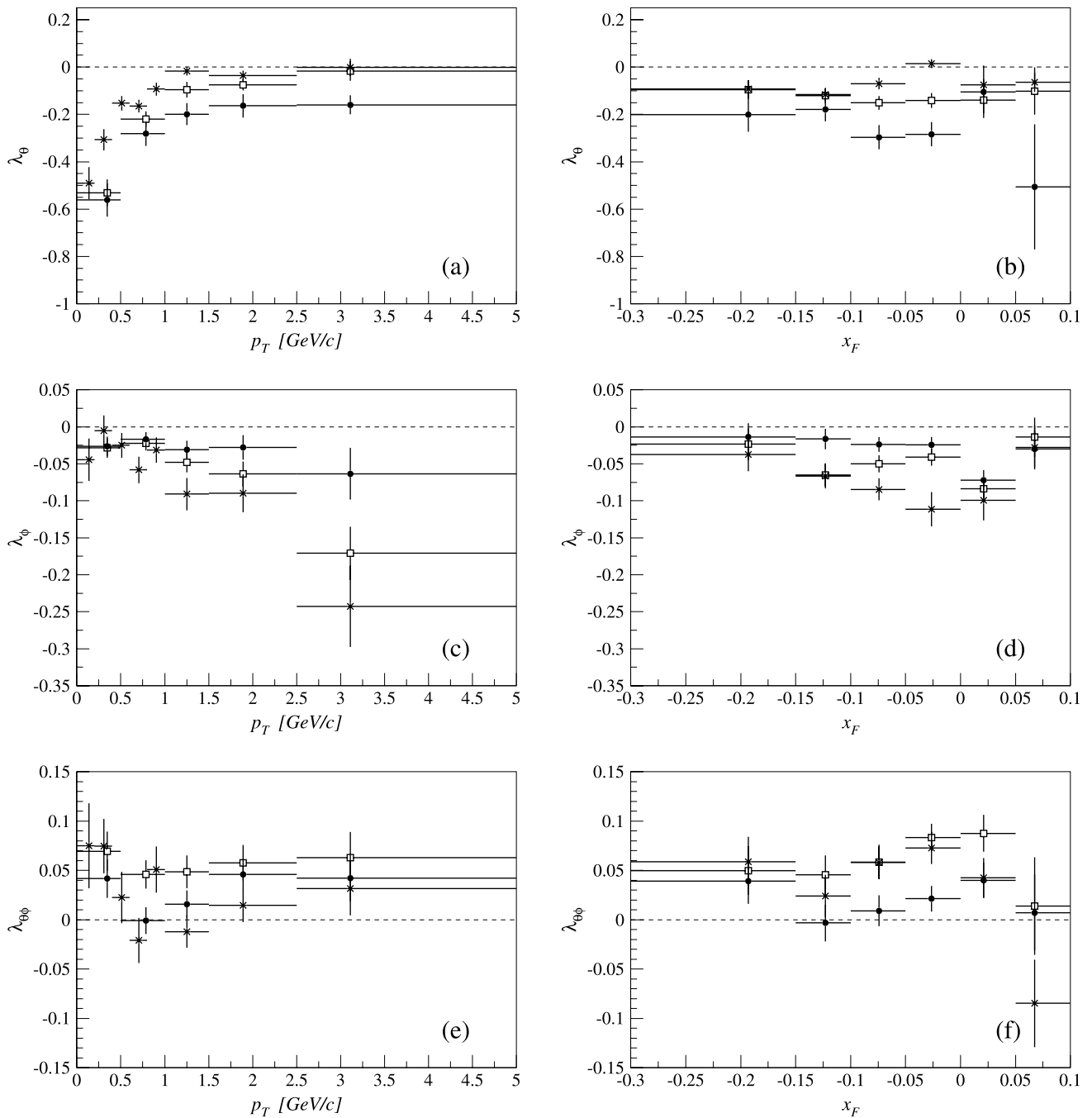
Fig. 3.2 The parameters \lambda_\theta (a, b), \lambda_\phi (c, d) and \lambda_{\theta\phi} (e, f) measured as functions of the average reconstructed p_T (left column) and x_F (right column). The results obtained in the Collins-Soper, Gottfried-Jackson and helicity frames are represented, respectively, by black cir-
