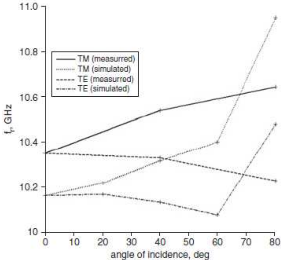
Fig. 3 Measured and simulated values of resonance frequency f_r against angle of incidence
