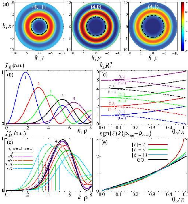
FIG. 2: (Color online) (a) Intensity distributions, Eq. (28), marked by quantum numbers (\ell, \sigma) for Bessel beams with \theta_0 = 3\pi/8 . The spin-dependent profiles are shown for \ell = 4 with \sigma = -1, 0 (scalar case), and 1. Dashed circles indicate the GO caustics (28). (b) Radial intensity profiles of the scalar ( \sigma = 0 ) or paraxial ( \theta_0 \rightarrow 0 ) Bessel beams I_{|\ell|} = J_{|\ell|}^2(\xi) . (c) The SOI splitting of the profile of the polarized non-paraxial Bessel beam I_{\pm 4}^{\sigma}(\xi) , Eq. (27), at different values of \theta_0 ; vertical lines indicate GO caustics (28), cf. (a). (d) The GO caustics (28) marked by \text{sgn}(\ell)(\ell, \sigma) as functions of \theta_0 . (e) The SOI splitting of the maxima of intensity (27) [cf. (c)] as dependent on \theta_0 , approaching the GO limit (28) at |\ell| \gg 1 .
