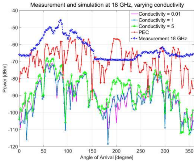
Fig. 7 Varying conductivity for simulation at 18 GHz
