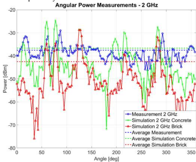
Fig. 5 Angular power distribution for 2 GHz
