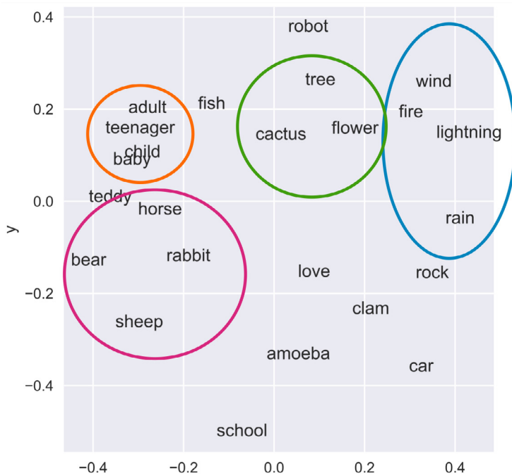
Figure 6: A multidimensional scaling (MDS) plot showing the distances between the 24 nouns, averaged over the 100 languages in the second half of the experiment. Two nouns are close in this plot if they tend to take the same noun-class marker within a language, and far apart if they tend to take different noun-class markers. Four animacy-related clusters (humans, plants, land animals, natural forces) have been circled for illustrative purposes.
