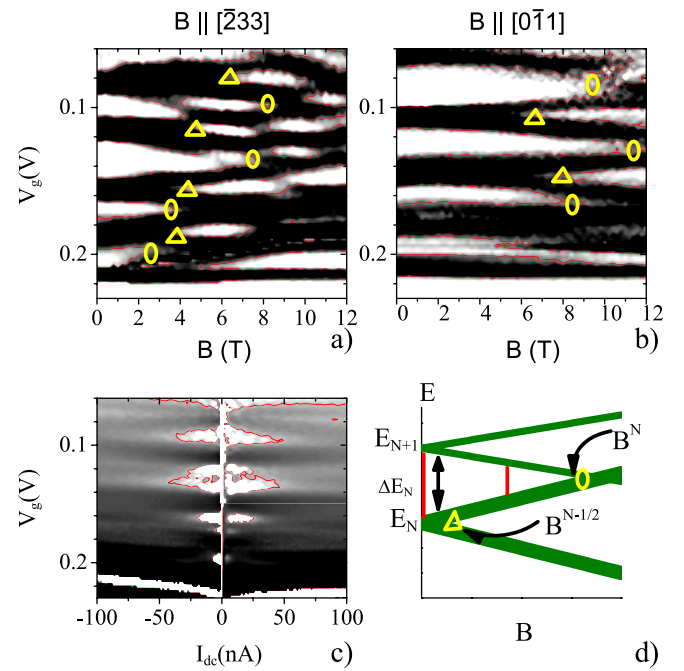
FIG. 3 (color online). (a),(b) Derivative of curves in Figs. 1(a) and 1(b), white regions correspond to the conductance plateaus. (c) Differential transresistance plotted in a logarithmic scale [from 0.01 k \Omega (white) to 0.2 k \Omega (black)] for the same sample at B = 0 . (d) Schematic of Zeeman splitting of energy levels.
