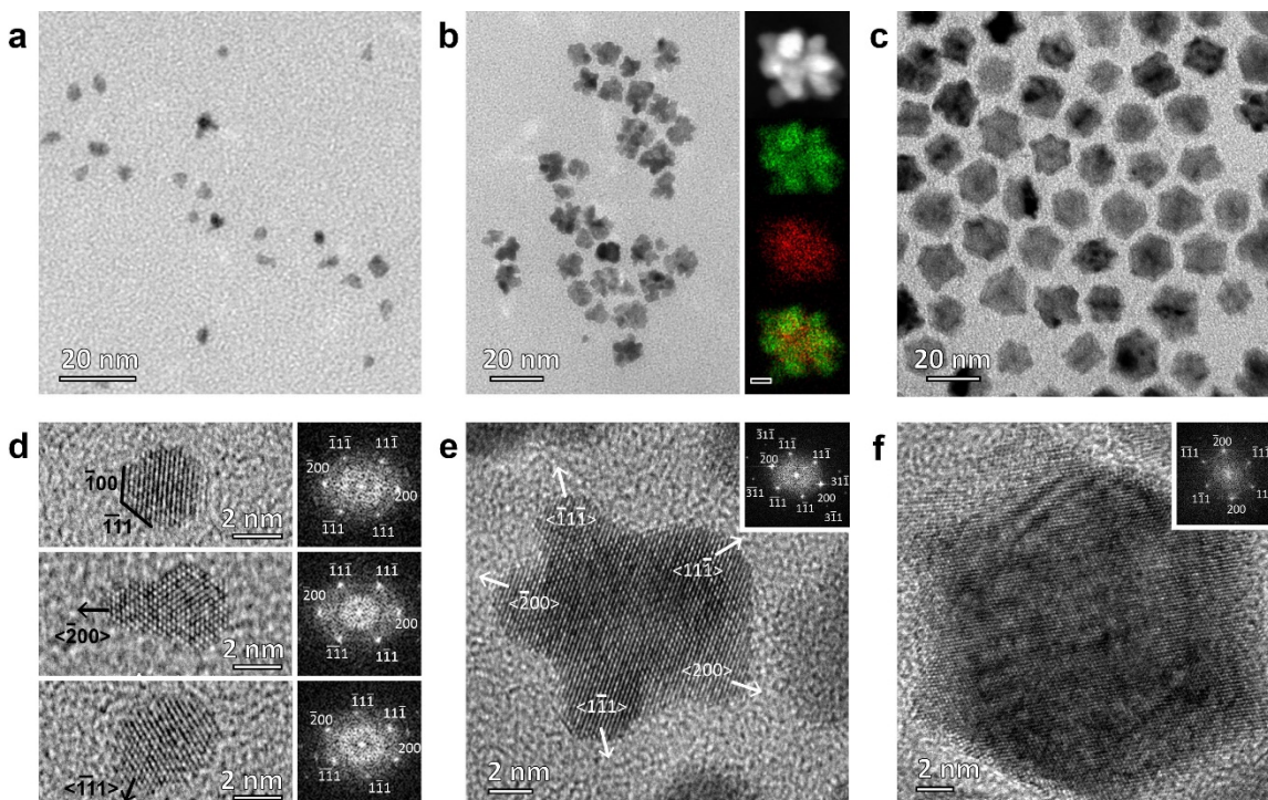
Figure 1. Formation process of the rhombic dodecahedra. TEM (a, b, and c) and corresponding HRTEM (d, e, and f) images of interim products obtained from the growth solution when its color is green, yellow, and brown respectively. HAADF-STEM and EDS elemental mapping images (b, right) of a typical particle in b: green is Pt and red is Ni, scale bar = 2 nm. FFTs of the corresponding HRTEM images (d, right; insets in e and f) indicate the growth directions of elongated nanoparticles and branched nanostructures. Moiré patterns (f) indicate the superimposition of two phases with different lattice constants present in the particle 24 .
