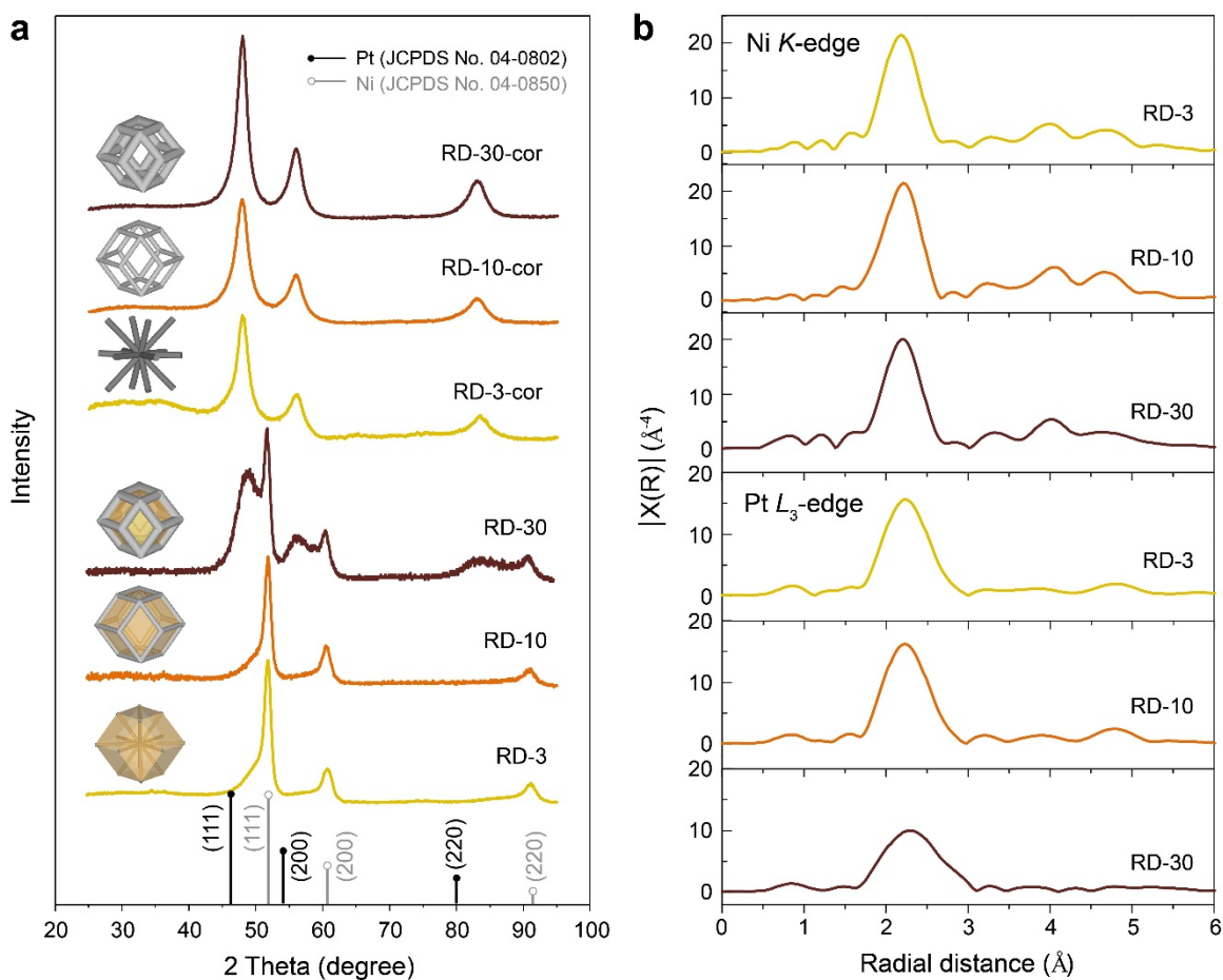
Figure 4. Structural evolution over time in Pt-Ni rhombic dodecahedra. Powder X-ray diffraction patterns of rhombic dodecahedra and their corresponding chemically corroded products (a). RD-3 and RD-10 show asymmetric diffraction peaks at lower 2\theta that indicate the co-existence of segregated Pt-rich phase. The asymmetric peaks split into two sets of diffraction patterns for RD-30, in which more Pt had grown on the edges. Ni K-edge and Pt L_3 -edge EXAFS spectra (b) of rhombic dodecahedra. RD-3 and RD-10 have similar EXAFS spectra due to their nearly identical bulk compositions, while RD-30 has lower intensity in its first-shell peaks at the Ni K-edge and Pt L_3 -edge due to its increased phase segregation and Pt enrichment.
