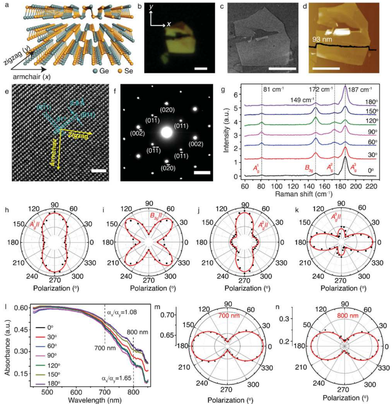
Figure 1. a) Schematic representation of the side view of the crystal structure of GeSe. b) Reflection microscope image of a typical exfoliated GeSe flake. x- and y-axes in the inset signify the reference axes. c) SEM image of the same flake. d) AFM image of the GeSe flake with the line profile in the inset shows that the flake is 93 nm thick and has an atomic smoothness. Scale bars are 5 \mu\text{m} . e) HRTEM image of the GeSe flake. Scale bar is 2 nm. f) Corresponding SAED pattern. Scale bar is 2 \text{nm}^{-1} . g) Raman spectra acquired in parallel polarization configuration from the GeSe flake for different polarization angles between 0° and 180° with respect to the x-axis. h–k) Polar plots of the Raman intensities of A_g^1 (81 \text{cm}^{-1} ), B_{3g} (149 \text{cm}^{-1} ), A_g^2 (172 \text{cm}^{-1} ), and A_g^3 (187 \text{cm}^{-1} ) Raman modes, respectively. Experimentally measured Raman intensities (data points) match well with the corresponding theoretical fits (red solid curves). l) Measured polarization-resolved absorption spectra for different linear polarization angles between 0° and 180°. m, n) Evolution of the measured absorbance (data points) as a function of the polarization angle at two different wavelengths of 700 and 800 nm. The red solid curves are the corresponding fits with the sinusoidal function.
