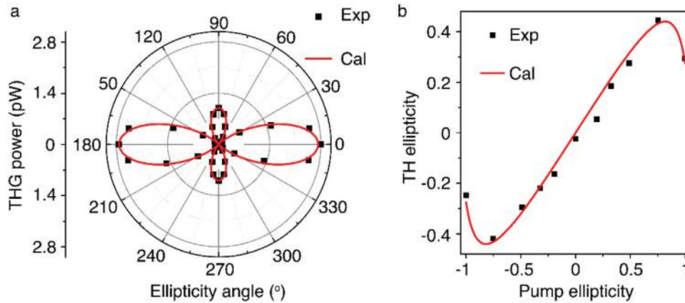
Figure 6. a) Dependence of the average THG power on the ellipticity angle of pump beam. 0° and 180° correspond to the linear polarization along the armchair direction; 90° and 270° correspond to the linear polarization along the zigzag direction; while 45°, 135°, 225°, and 315° correspond to the circular polarization. b) Evolution of the TH ellipticity as a function of the ellipticity of pump beam.
