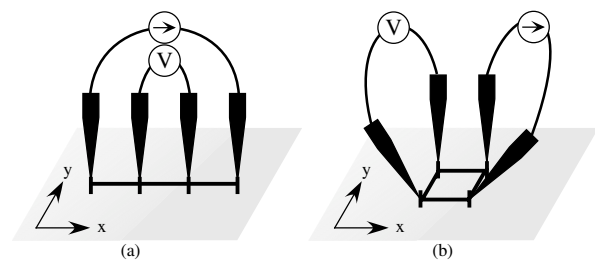
FIG. 1. Schematic drawings of the four-point probe method in (a) linear and (b) square arrangements. The probes are equidistant from each other. Current and voltage probes are shown.
