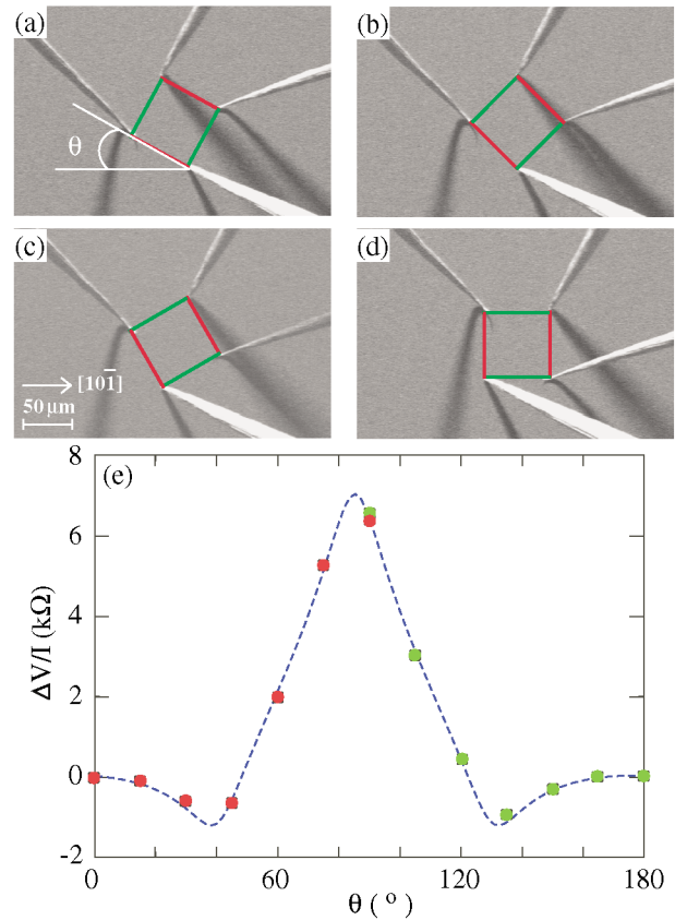
FIG. 4 (color). SEM images of rotational square micro-4PP measurements with 60 \mu\text{m} probe spacing, at (a) \theta = 30^{\circ} , (b) 45^{\circ} , (c) 60^{\circ} , and (d) 90^{\circ} . (e) Angle dependence of the measured resistance \Delta V/I of the single-domain 4 \times 1 -In surface. Experimental data are fitted by Eq. (3).
