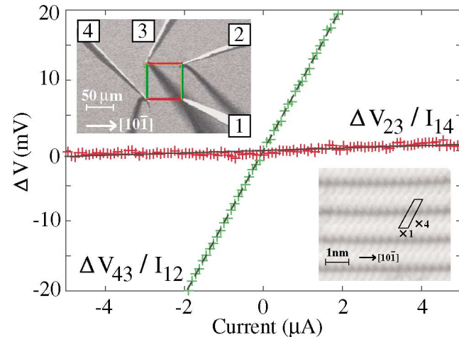
FIG. 2 (color). I - V curves of a single-domain Si(111) 4 \times 1 -In surface measured by square micro-4PP method with the probe spacing (a side of the square) of 60 \mu\text{m} . The red and green colors correspond to the measurements of \Delta V_{23}/I_{14} and \Delta V_{43}/I_{12} , respectively. The upper left inset is a SEM images of the probes. The In chains were parallel to the [10\bar{1}] direction, horizontal direction in this image, which was determined by RHEED. The lower right inset is a STM image of the 4 \times 1 -In surface, separately taken by another single-tip STM.
