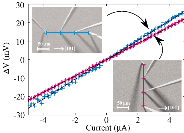
FIG. 3 (color). I - V curves of a single-domain 4 \times 1 -In surface measured by linear micro-4PP method with 60 \mu\text{m} probe spacing. The blue and purple colors correspond to the measurements parallel and perpendicular to the In chains (horizontal direction in these SEM images), respectively.
