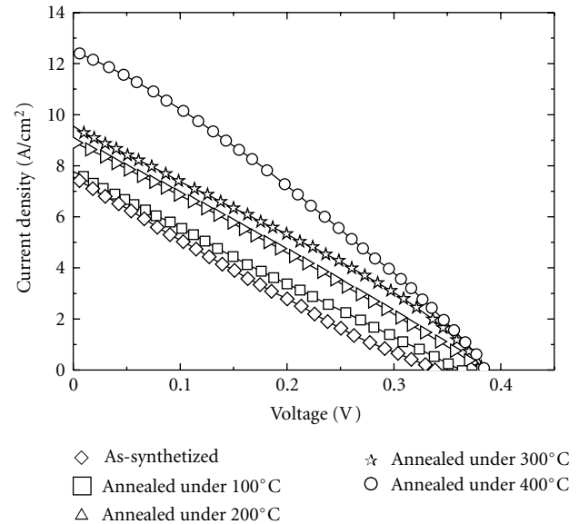
FIGURE 6: I-V curves for the solar cells assembled using CdSe-TiO 2 nanostructures annealed under different temperatures.
