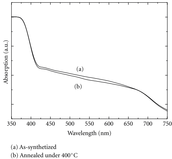
FIGURE 5: Optical absorption spectra of nanorod arrays with and without annealing treatment.
