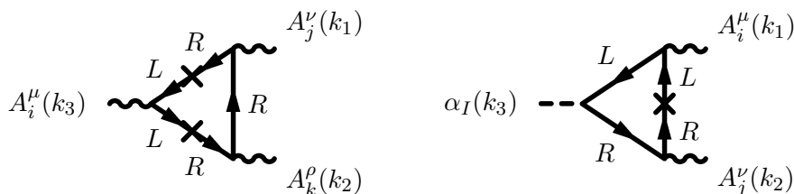
Figure 1: The first diagram is one of the twelve diagrams which contribute to the GCS terms. The second is one of the six diagrams which contribute to the axionic couplings. Both are obtained by integrating out heavy fermions.
