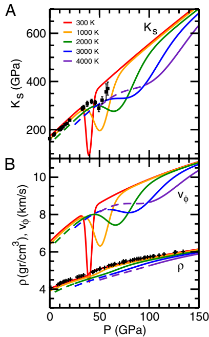
Fig. 2. Pressure dependence of the calculated adiabatic bulk modulus (A), K_S , and bulk wave velocity (B), V_\phi and density, \rho , of Mg_{1-x}Fe_xO ( x = 0.1875 ) along several isotherms. Full (dashed) lines correspond to results within (outside) the (P and T) regime of validity of the QHA (1, 24). Experimental data for K_S on a sample with X_{Fe} = 0.06 (10) is shown in A. The calculated anomaly is approximately 3 times larger than the observed one. Crosses on B are experimental data at 300 K on a sample with X_{Fe} = 0.17 (15).
