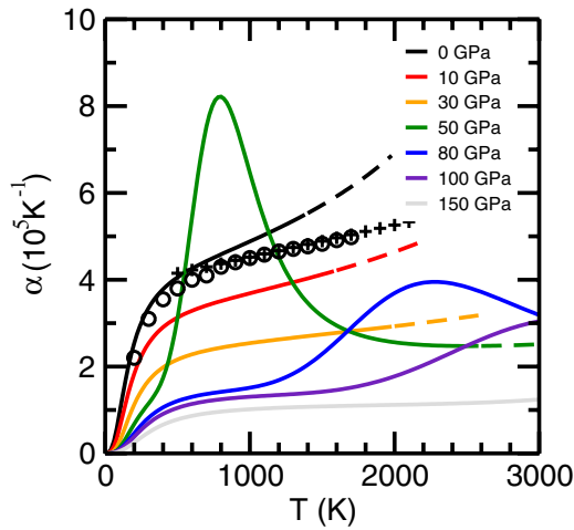
Fig. 1. Thermal expansivity of Fp along several isobars. Full (dashed) lines correspond to results within (outside) the (P and T) regime of validity of the QHA (1, 24). Circles and crosses are experimental values at 0 GPa for Mg_{1-x}Fe_xO with x = 0.0 (22) and x = 0.36 (23), respectively.
