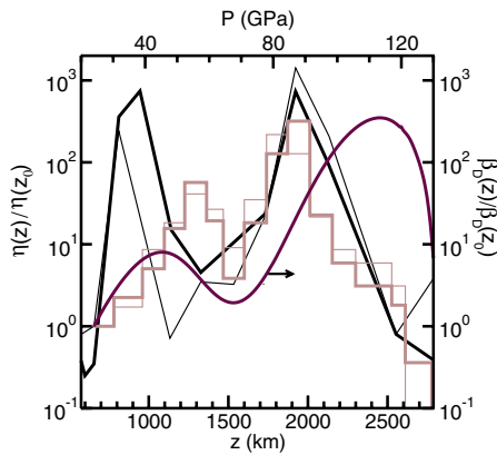
Fig. 4. Viscosity of ferropericlase along a mantle geotherm (29) compared with mantle viscosity models (36, 37). Thin and thick black lines (37) were derived from convection related data extracted from geoid inversion and 2 distinct tomography models, refs. 47 and 48, respectively. Thin and thick light-brown lines (37) included also glacial rebound data in the derivation of the viscosity models. The tomography models were the same as those used in ref. 37. Thick maroon line is the relevant property of Fp computed in the MS state. \beta_D(z) is the contribution of the dilatational component of the activation energy, G_D(z) , to \eta_{Fp}(z) ( \delta = 0 only).
