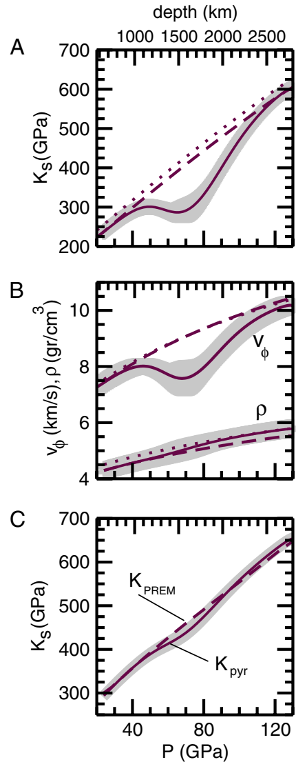
Fig. 3. Properties of Mg_{1-x}Fe_xO ( x = 0.1875 ) along a lower mantle geotherm (29). (A) Adiabatic bulk modulus, K_S ; (B) bulk velocity, V_\phi , and density, \rho ; and (C) bulk modulus of an aggregate with pyrolite composition, K_{pyr} , compared with PREM's (30) bulk modulus, K_{PREM} . In A and B, full, dashed, and dotted lines correspond to properties computed in the MS, HS, and LS states, respectively. Shaded regions represent the uncertainties caused mainly by the uncertainty in the computed enthalpies of HS and LS states (see SI Text ) and spin cross-over pressure at T = 0 K.
