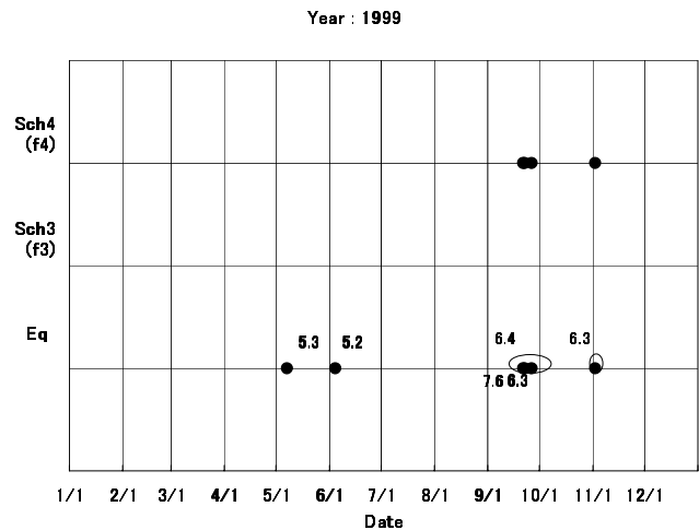
Fig. 2. One-year (1999) summary of SR observations in Nakatsugawa and anomalous SR behaviors in possible association with two large land earthquakes in Taiwan. Dots on Sch4 mean that an anomaly is taking place at the fourth SR mode, and no dots on Sch3 mean that there is no effect at the third SR mode. An earthquake with a circle indicates the land earthquake, while an earthquake without a circle means that it occurs in the sea.
