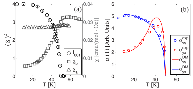
FIG. 8. (Color online) (a) The scaled intensity of the 001 peak measured on RITA-II and the molar susceptibilities for fields along a and b from Ref. [49]. (b) The measured ME coefficients \alpha_{xy} and \alpha_{yx} taken from Ref. [5] compared to the calculated temperature dependencies in arbitrary units.
