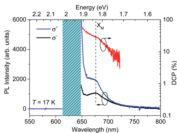
Fig. 3 Helicity resolved PL spectra and degree of polarization (DCP) obtained from the \text{MoS}_2/\text{WS}_2 HS with 633 nm, circularly polarized ( \sigma^+ ) excitation at T = 17 K. The shaded blue region indicates the stopband of the filter used to block the laser light from reaching the detector.
