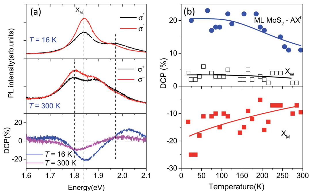
Fig. 2 (a) Helicity resolved PL spectra obtained from the \text{MoS}_2/\text{WS}_2 HS with 532 nm, circularly polarized ( \sigma^+ ) excitation at T = 16 K (top panel) and T = 300 K (middle panel). Degree of polarization (DCP) at T = 16 K and T = 300 K (bottom panel) obtained with 532 nm, \sigma^+ excitation of the \text{MoS}_2/\text{WS}_2 HS. (b) DCP near the X_M and X_W peaks, at different temperatures, obtained with 532 nm, \sigma^+ excitation of the \text{MoS}_2/\text{WS}_2 HS. The DCP data corresponding to the charged exciton ( \text{AX}^- ) in ML- \text{MoS}_2 are also shown in the top panel. The solid lines are a guide for the eye.
