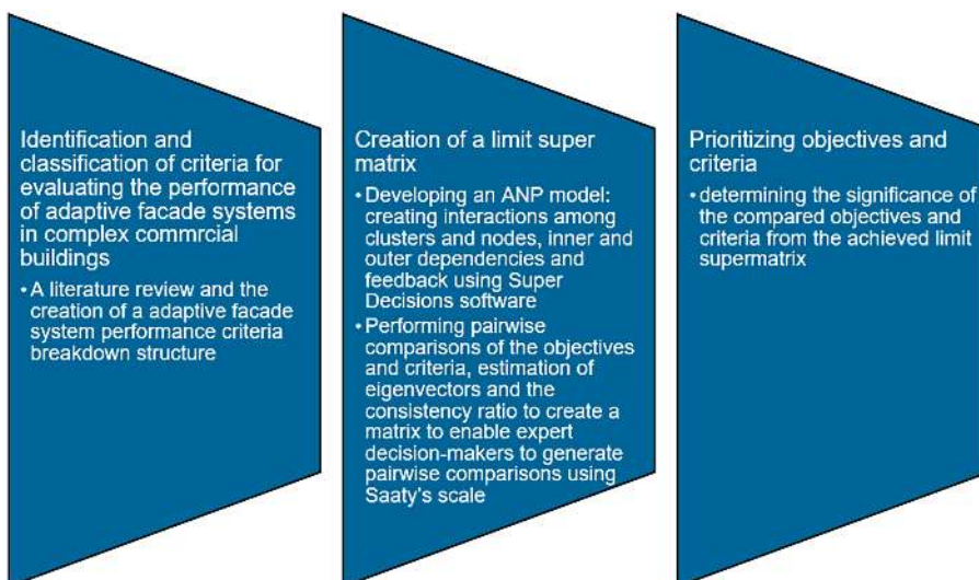
Figure 2. Implementation of ANP model for evaluation of the performance of adaptive façade systems in complex commercial buildings
