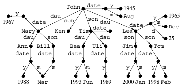
Figure 1. A database
