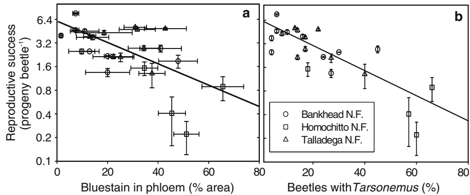
Fig. 4 Relationships between per capita reproductive success of D. frontalis and a percent bluestain ( O. minus ) in phloem ( y = 1.68 - 0.03x , P < 0.01 , r^2 = 0.37 ) and b percent of beetles carrying phoretic mites ( Tarsonemus ; y = 1.83 - 0.037x , P < 0.01 ,
