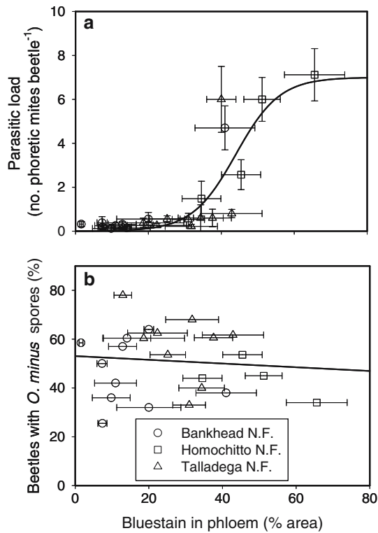
Fig. 5 Relationships between O. minus in phloem and a phoretic mites/beetle ( y = 7/e^{-(x-44)/6} ), P < 0.01 , r^2 = 0.74 ) and b percent of adult D. frontalis (phoretic mites removed) with O. minus spores on their exoskeleton ( y = 53 - 0.048x , P < 0.68 , r^2 = 0.00 ). Each symbol represents one infestation within the Bankhead (circle), Homochitto (square box), or Talladega (triangle) National Forests ( \pm SE based on five trees per infestation)
