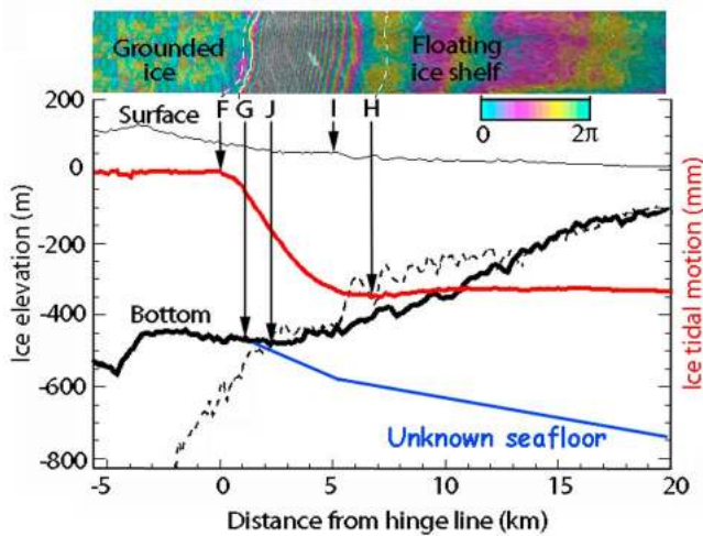
Figure 1. Grounding zone of Petermann Glacier, Greenland, with the limit of tidal flexing (F), the grounding line (G), the line of first hydrostatic equilibrium (J), the break in surface slope (I), the maximum extent of the flexure zone (H), ice surface elevation above mean sea level from laser altimetry (thin black line), bed topography from radio echo sounding (thick black line), bed depth calculated from hydrostatic equilibrium (dashed black line), the unknown seafloor (over-deepening likely exceeds 800 m) and tidal flexing measured with ERS-1 DInSAR in millimeter of vertical motion (red thick line). The color inset on top shows the DInSAR interferometric fringes, color coded from 0 and 2\pi , from blue to yellow, red and blue, and delineates F (dotted white line near G), G (white line), and H (dotted white on floating ice). Ice flows from left (grounded ice) to right (floating ice).
