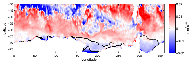
Fig. 3. Annual mean buoyancy flux from a state estimate that combines 3 yr of available observations with an ocean model (26). The black line denotes the 70% quantiles of annual mean sea ice concentration, essentially the area of the ocean covered by ice 70% of the time. The change in sign of the buoyancy flux just north of the Antarctic continent is roughly collocated with the 70% quantile of sea ice coverage.
