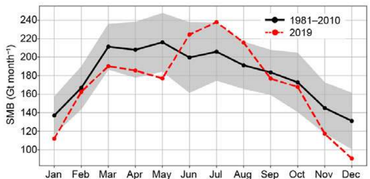
Fig. 6.6. Seasonal cycle of (grounded) AIS integrated surface mass balance (SMB) according to MERRA-2 for 2019 (red) and 1981–2010 (black line = mean, gray shading: std. dev.).
