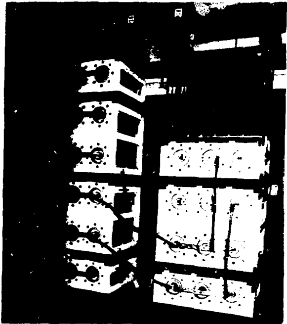
Fig. 9. Partially assembled Marx generator with capacitors in racks.
