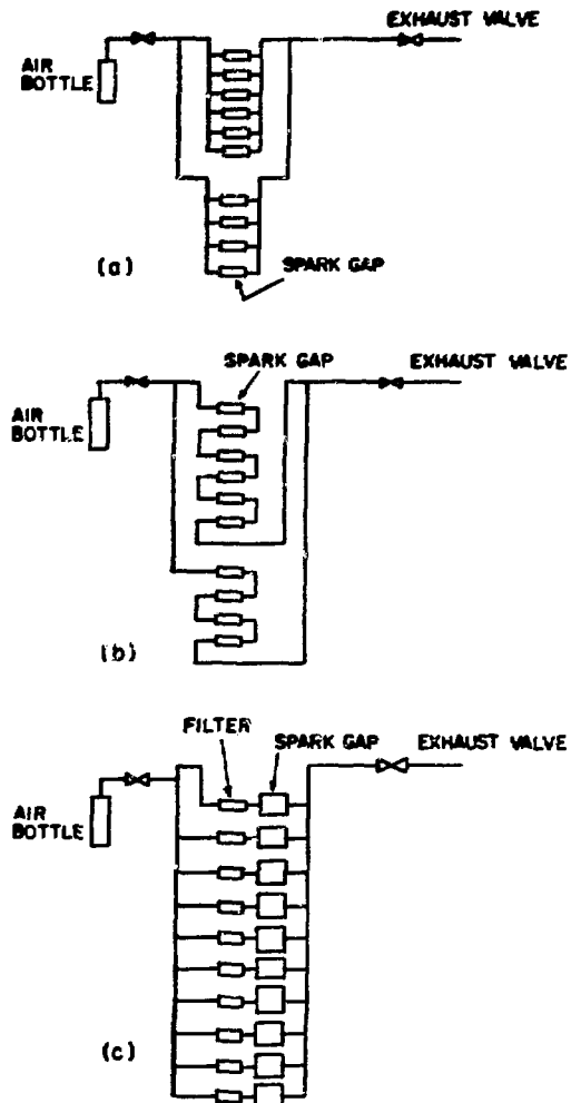
Fig. 11. Airflow systems.
