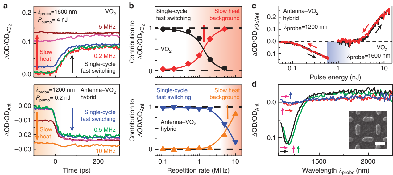
Figure 2 Contributions of the fast picosecond and slow thermal response to the optically driven IMT in VO 2 and antenna–VO 2 hybrids. (a) Time-dependent response of VO 2 (top, \lambda_{probe} = 1600 nm) and antenna array with L_v = L_h = 210 nm (bottom, \lambda_{probe} = 1200 nm) for repetition rates of 0.2 MHz (red), 0.5 MHz (green), 1 MHz (blue), 2 MHz (magenta), 5 MHz (brown) and 10 MHz (orange). The effect before 0 ps corresponds to a slow heat background, with the step at 0 ps corresponding to single-cycle fast switching caused by picosecond phase transition. Pump energy P_{pump} for the VO 2 film, 4 nJ; for the antenna array, 0.2 nJ. (b) Relative contributions of single-cycle fast \Delta OD_{fast}/\Delta OD and slow heat background \Delta OD_{slow}/\Delta OD (see text) obtained from the time traces in a . The antenna array shows \times 5 increased operating speed for single-cycle fast switching compared with pure VO 2 . (c) Phase-change modulation \Delta OD/OD versus optical pulse energy at \lambda_{probe} = 1200 nm for the antenna array and at \lambda_{probe} = 1600 nm for the VO 2 film, both at 0.1 MHz. The blue shaded region indicates the damage threshold for the antenna array. (d) Differential nonlinear response spectrum \Delta OD/OD_{Ant} for an antenna array with L_v = L_h = 210 nm, for different combinations of pump (magenta arrows) and readout (black/red arrows, horizontal, green/blue arrows, vertical) polarizations, at a temperature of 50 °C, 0.1 MHz pump laser repetition rate, and 0.6 nJ pump energy.
