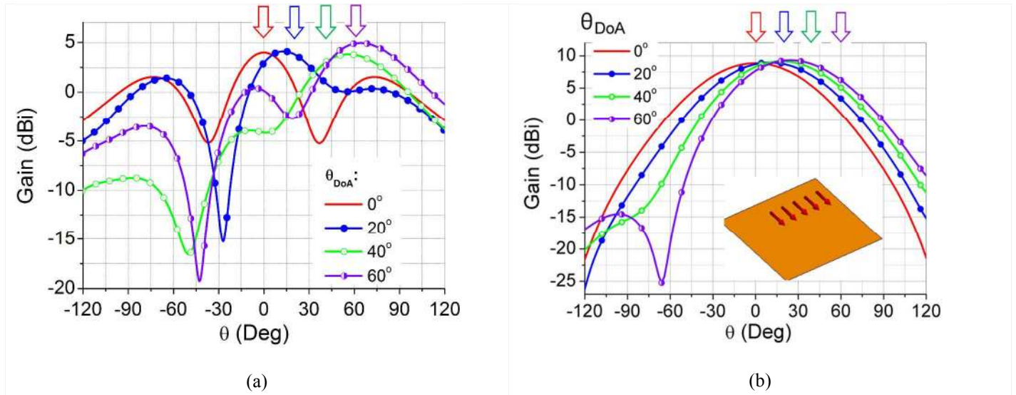
Fig.3. Simulated retrodirected radiation pattern at 2.4GHz in y - z plane generated by (a) resonance antenna array (a) and a counterpart array composed of Hertzian dipole sources located in the positions corresponding to the antennae centers, (b). The phase excitations of the Hertzian array are the conjugate of the incident field phase in the dipoles' positions. No scattering/EM coupling is present in the Hertzian dipole array case. Arrows on top of the graphs show the DoA. The simulated return loss fractional bandwidth of the resonance antenna elements is \sim 3\% at -10 dB level, array elements are center-loaded with 10\Omega lumped loads [18].
