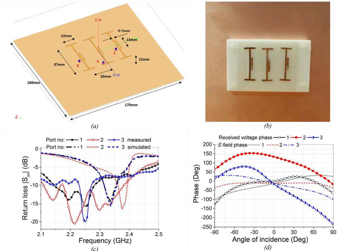
Fig.7. Planar 3-element antenna array FEKO simulation model(a) and fabricated prototype (b); simulated and measured antenna return loss (c) and measured RX voltage across the ports 1-3 at 2.25GHz, (d). In (d) the simulated phase of the incident field in the locations corresponding to the antenna element centers is also shown for comparison.
