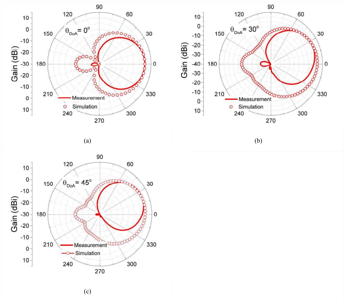
Fig.8. Retro-directive radiation patterns generated by a 3-element array at 2.25GHz for DoA (a)0, (b)30 and (c)45 degrees. Solid line – measurements, dotted line - simulations
