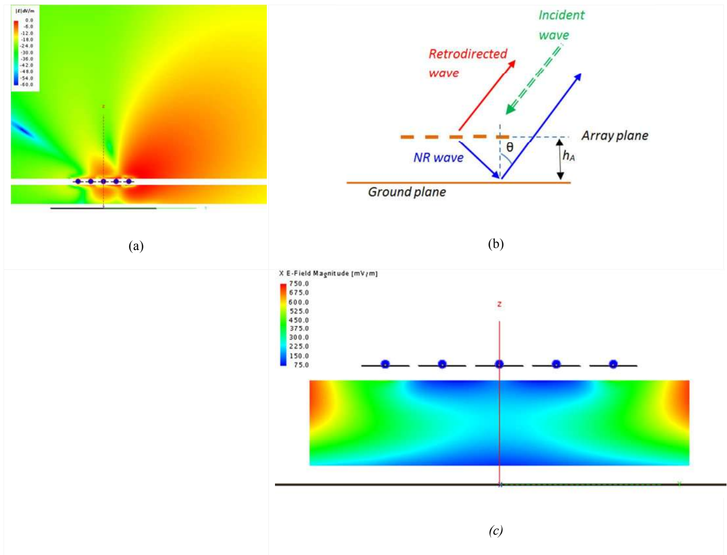
Fig.4. (a) Simulated retrodirected normalized E-field pattern at 2.4GHz in y-z plane generated by a resonance antenna array for the DoA 40^\circ . (b) Ray representation of the propagating EM waves radiated by the antenna array. (c) Near E-field between the 5-element antenna array and a flat metal ground plane with \lambda/4 vertical offset distance, full-wave FEKO simulation. The antenna array in the receive mode, DoA = 0^\circ .
