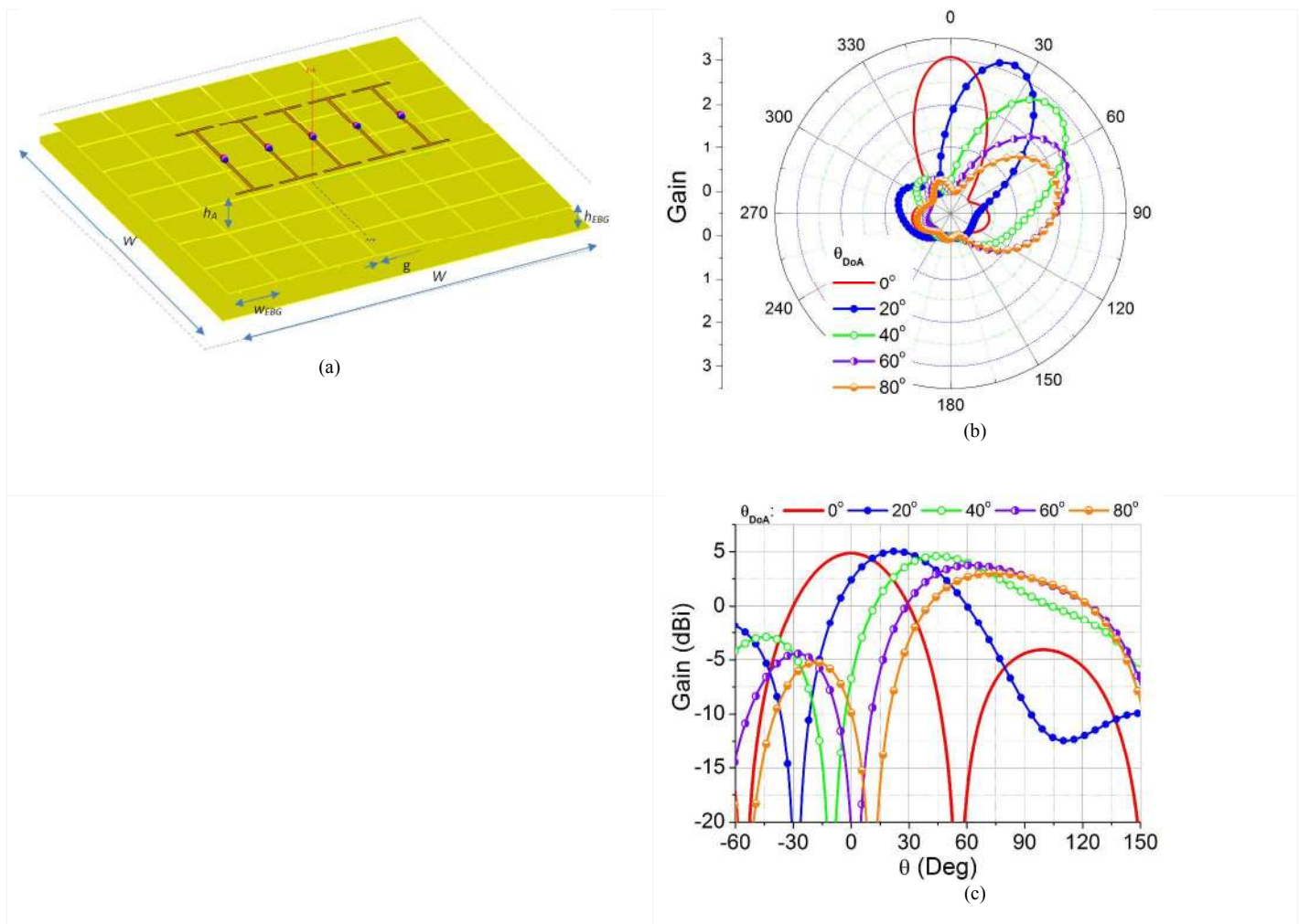
Fig.5. (a) 5-element planar antenna array with the EBG ground plane. The dimensions of the antenna array are the same as in Fig. 3(a): l_a = 0.3\lambda , d_y = 0.12\lambda . The ground plane parameters are W = 1.0\lambda , the square patch mushroom type EBG has dimensions w_{EBG} = 0.13\lambda , h_{EBG} = 0.05\lambda , g = 0.004\lambda , and h_A = 0.125\lambda , \lambda = 0.125\text{m} ; (b) Simulated polar plot of the retrodirective patterns in the yz plane (in terms of absolute gain) for various DoA; (c) Retrodirective patterns logarithmic gain in the angular range close to the radiation pattern maximum. The simulated return loss fractional bandwidth of the resonance antenna elements is \sim 4.5\% at -10\text{dB} level, array elements are center-loaded with 10\Omega lumped loads [18].
