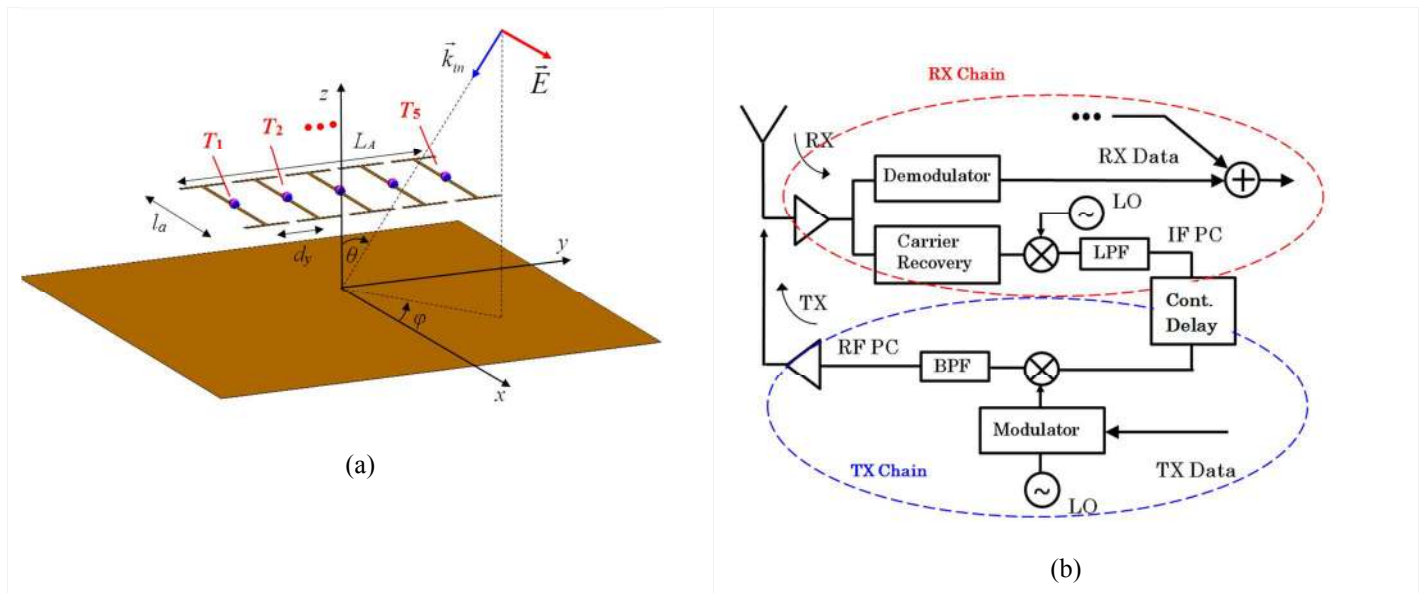
Fig.1. (a) A simulation model of an ultra-compact retrodirective antenna array illuminated by a linearly x -polarized monochromatic PW. The antenna array characteristic size L_a \sim N d_y \sim 0.5\lambda , N is a number of antenna elements, the inter-element spacings d_y are of order of 0.1\lambda . T_m , m=1,2,\dots,N are the PC antenna ports. The antennas are end-loaded to ensure electric
