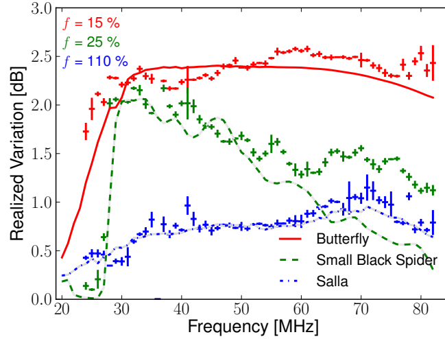
Figure 21: The measured galactic variation for the three antennas as a function of frequency here indicated with the bar symbols. The continuous lines give the expected variation from simulations as in Fig. 20 but with a noise power added that is constant in frequency. The percentages denote the strength of the added noise floor relative to the maximum signal expected from the galactic background.
