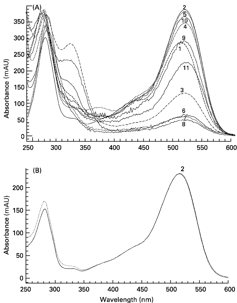
Fig. 2. UV-visible absorption spectra of anthocyanins in human urine and serum samples post-consumption of chokeberry extract monitored at 525 nm by HPLC–diode array detector (DAD). (A), Typical UV-visible absorption spectra of individual peaks in human urine and serum samples post-consumption of the extract; (B), UV-visible absorption spectra of peak 2 (—) and cyanidin 3-galactoside standard (- -). HPLC chromatogram of urine and serum samples are given in Fig. 1. Urine and serum concentrations of each compound represented by peaks 1 to 11 are given in Tables 1 and 2, respectively. Urine and serum concentrations of anthocyanins were determined using HPLC–DAD and quantified in relation to known concentrations of a cyanidin 3-galactoside standard.
