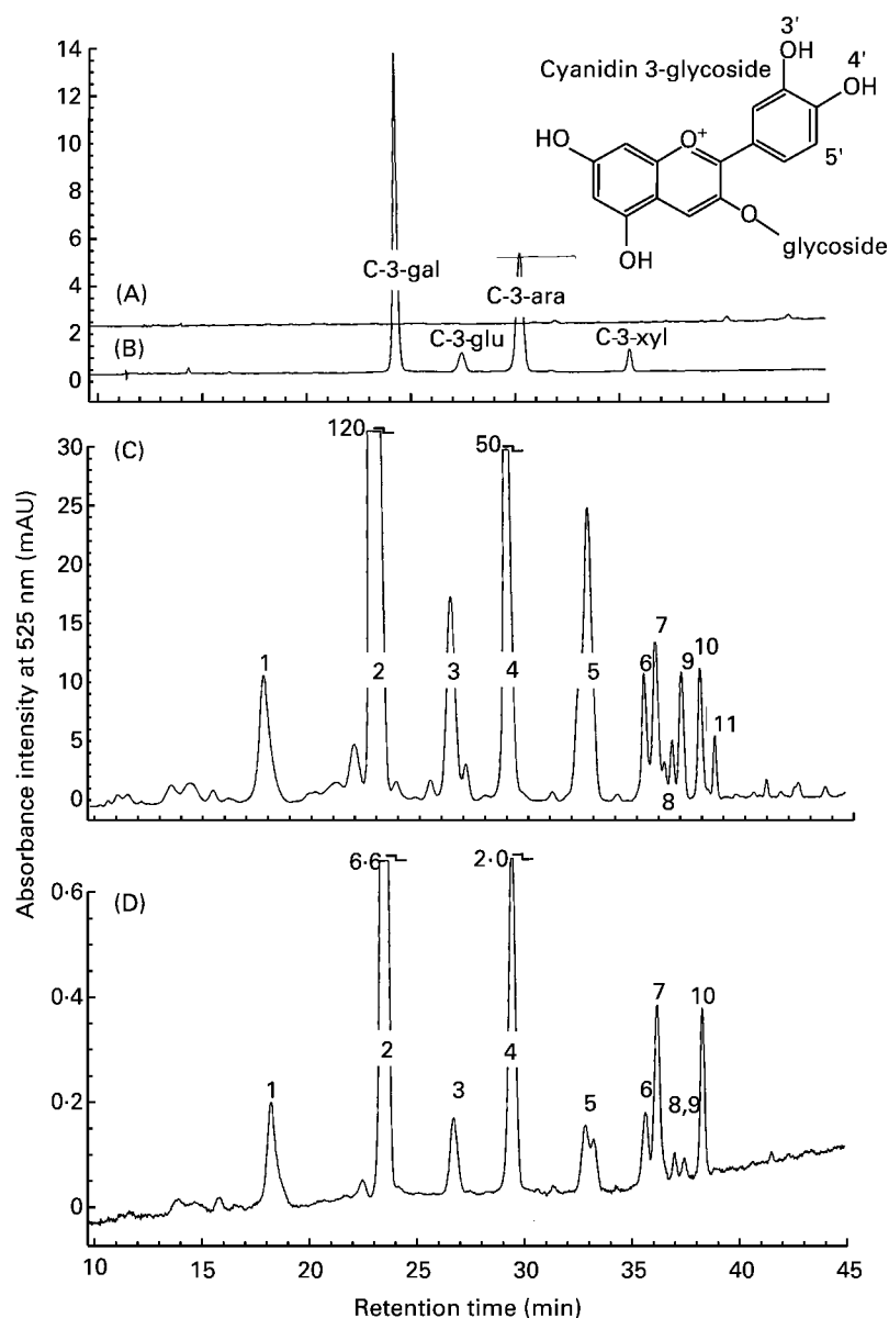
Fig. 1. Anthocyanins in chokeberry extract, and human urine and serum post-consumption of extract. (A), Chromatogram of baseline urine sample; (B), chromatogram of chokeberry extract; (C), chromatogram of 5 h urine sample; (D), chromatogram of 2 h serum sample; C-3-gal, cyanidin 3-galactoside; C-3-glu, cyanidin 3-glucoside; C-3-ara, cyanidin 3-arabinoside; C-3-xyl, cyanidin 3-xyloside. HPLC analysis was as outlined on p. 934. Identification of chokeberry anthocyanins was based on that of known standards. When standards were not available identification was based on retention times and spectral data from the literature (Chandra et al. 2001). Urine and serum concentrations of each compound represented by peaks 1 to 11 are given in Tables 1 and 2, respectively. Urine and serum concentrations of anthocyanins were determined using UV-visible HPLC and quantified in relation to known concentrations of a C-3-gal standard.
