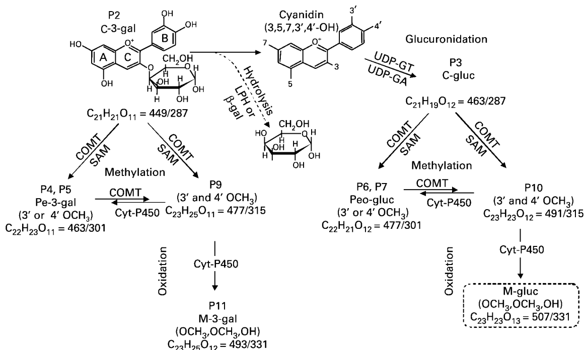
Fig. 3. Proposed pathway for the formation of anthocyanin metabolites in human urine and serum post-consumption of cyanidin 3-glycosides. P, peak; C-3-gal, cyanidin 3-galactoside; C-gluc, cyanidin glucuronide; M-3-gal, malvidin 3-galactoside; M-gluc, malvidin glucuronide; Peo-3-gal, peonidin 3-galactoside; Peo-gluc, peonidin glucuronide; COMT, catechol-O-methyltransferase; SAM, S-adenosyl methionine; LPH, lactase–phlorizin hydrolase; \beta -gal, \beta -galactosidase; UDP-GT, uridine diphosphate glucuronosyltransferase; UDP-GA, UDP-glucuronic acid; Cyt-P450, cytochrome P450. Molecular weights were obtained by MS (as outlined on p. 934). Identification was based on relative polarity (retention time), MS, and UV-visible data (as outlined on p. 934 and Table 1) and compared with those of known standards (Table 3). For an HPLC chromatographic plot of individual peaks, see Fig. 1. The circled metabolite is proposed but not identified. P1 and P8 are not illustrated as there were insufficient data available to elicit a potential structure. P9 and P10 have not been named as no anthocyanins of comparable structure have been reported to date.
