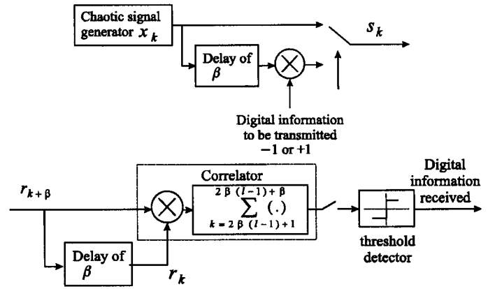
Fig. 3. Block diagram of a noncoherent DCSK system: (a) transmitter; (b) receiver.
