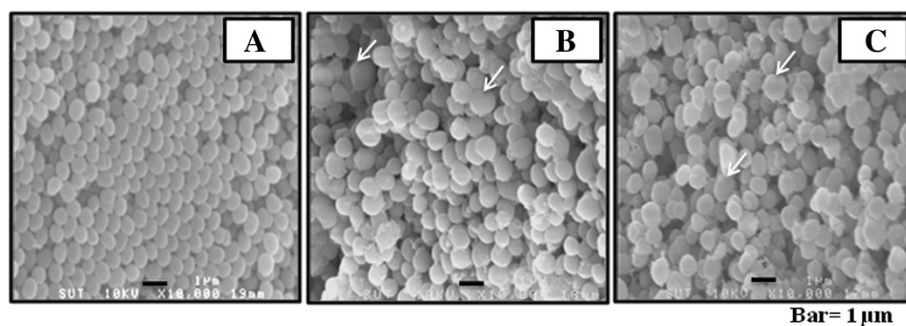
Figure 2 Scanning electron micrograph of S. epidermidis treated with A. crassna leaves extract. Cells were treated as described in Material and Method. The swollen cells (arrows) were observed after treated for 24 h with vancomycin (B) and the extract (C), compared with regular shape of control (A). Enlargement: \times 10000 .
