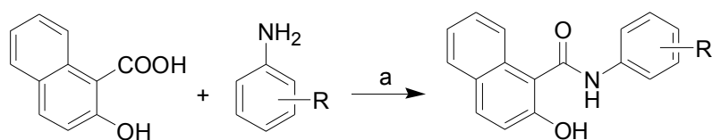
Scheme 1. Synthesis of ring-substituted 2-hydroxynaphthalene-1-carboxanilides 1–8c .
