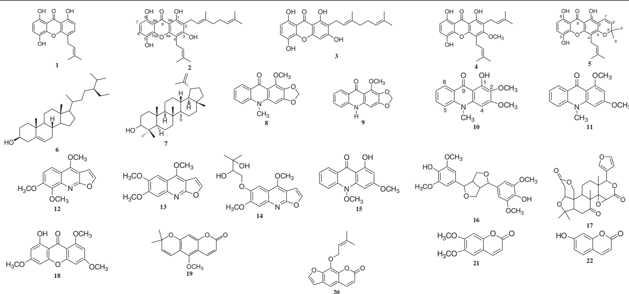
Figure 1 Chemical structures of compounds isolated from the stem bark of Garcinia nobilis (1-5), Orcia suaveolens woods (6-11) and roots (12-17), and the stem back of Balsmocitrus camerunensis (18-22). Caroxanthone (1), 4-prenyl-2-(3,7-dimethyl-2,6-octadienyl)-1,3,5,8-tetrahydroxanthone (2), smeathxanthone A (3), 8-hydroxycudraxanthone G (4), morusignin I (5), stigma-5-en-3-ol (6), lupol (7), evoxanthine (8), norevioxanthine (9), 1-hydroxy-2,3-dimethoxy-10-methylacridone (10), 1,3-dimethoxy-10-methylacridone (11), skimmianine (12), kokusaginine (13), monrifoline (14), 1-hydroxy-4-methoxy-10-methylacridone (15), syringaresinol (16), limonin (17), 1-hydroxy-3,6-dimethoxy-8-methylxanthone (18), xanthoxyletin (19), imperatorin (20), 6,8-dimethoxycoumarin (21), umbelliferone (22).
