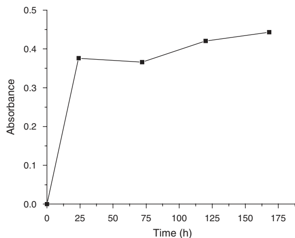
Fig. 1. Intensity absorbance of the plasmon resonance (440 nm) in function of time of reaction in an aqueous solution of 10 -3 M AgNO 3 with the fungal filtrate.
