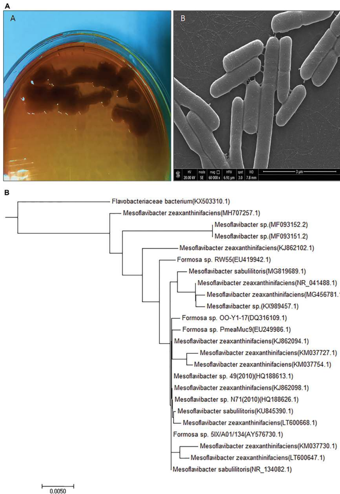
FIGURE 1 | Newly isolated exopolysaccharide producing and hypersaline bacterial strain information (A) Mesoflavibacter zeaxanthinifaciens purified culture on solid agar Zobell's medium plate and scanning electron microscopy image. (B) Phylogenetic tree of Mesoflavibacter zeaxanthinifaciens created by a neighbor-joining scheme based on accession number of gene sequences.
